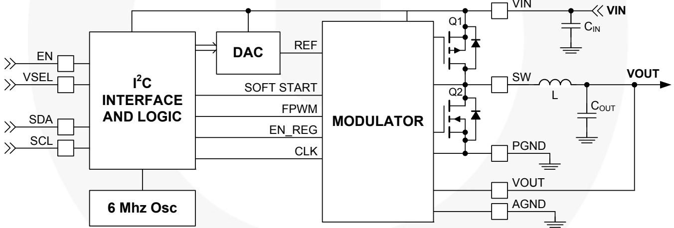
Figure 3 Block Diagram
