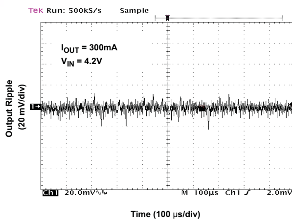
Figure 20. Output Ripple
