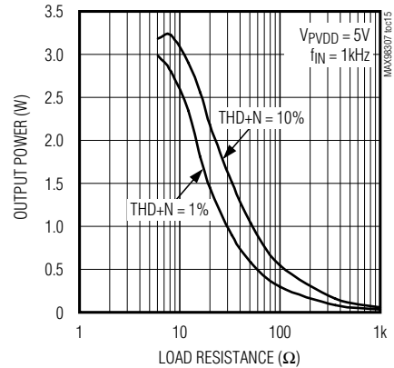
OUTPUT POWER vs. LOAD RESISTANCE (MAX98307)
