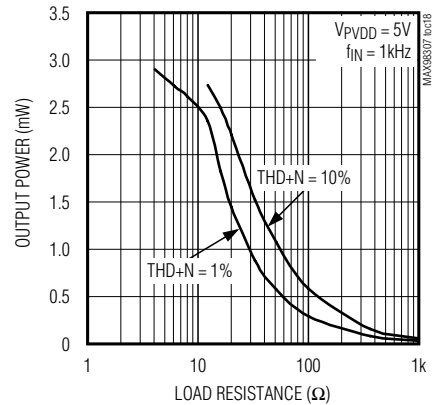
OUTPUT POWER vs. LOAD RESISTANCE (MAX98308)
