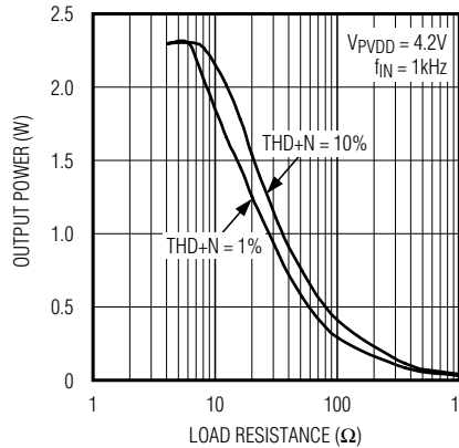
OUTPUT POWER vs. LOAD RESISTANCE (MAX98307)
