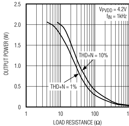
OUTPUT POWER vs. LOAD RESISTANCE (MAX98308)
