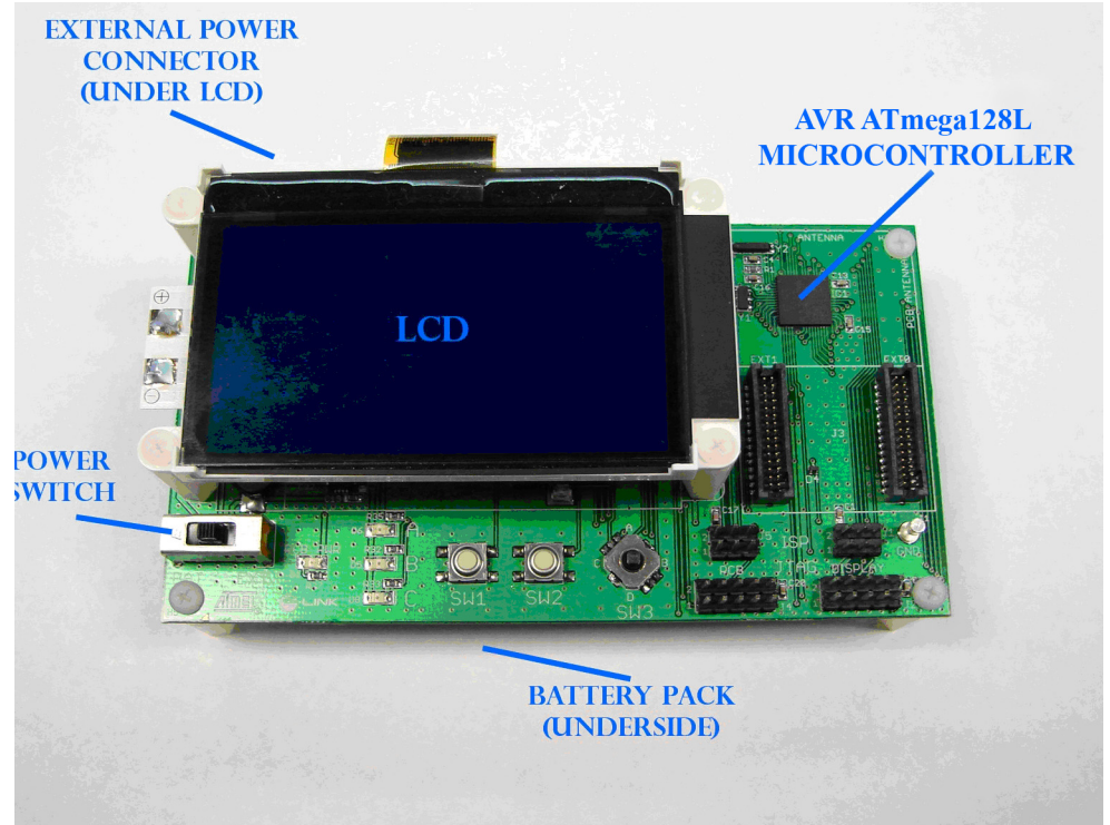
Figure 3-2. Key Components of the Display Board
