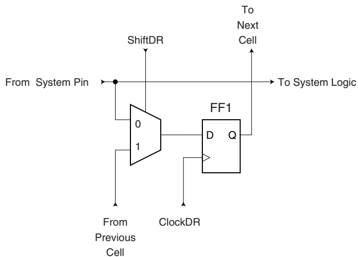
Figure 28-4. Observe-only Cell
