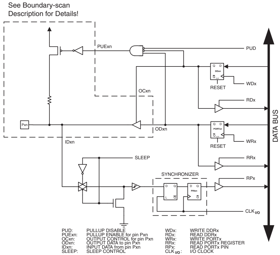
Figure 28-3. General Port Pin Schematic Diagram
