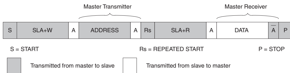
Figure 24-18. Combining Several TWI Modes to Access a Serial EEPROM
