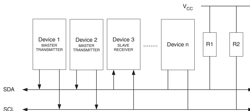
Figure 24-19. An Arbitration Example
