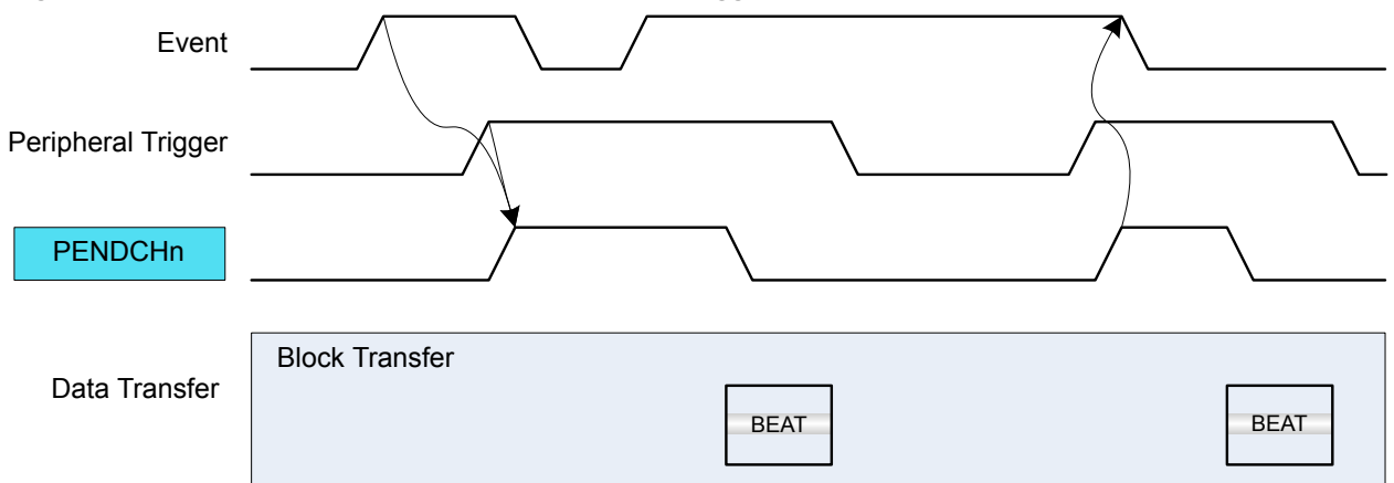
Figure 26-13. Conditional Event with Beat Peripheral Triggers
