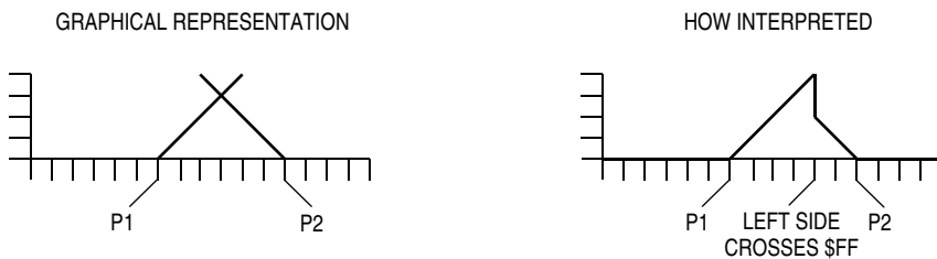
Figure 9-7. Abnormal Membership Function Case 2
