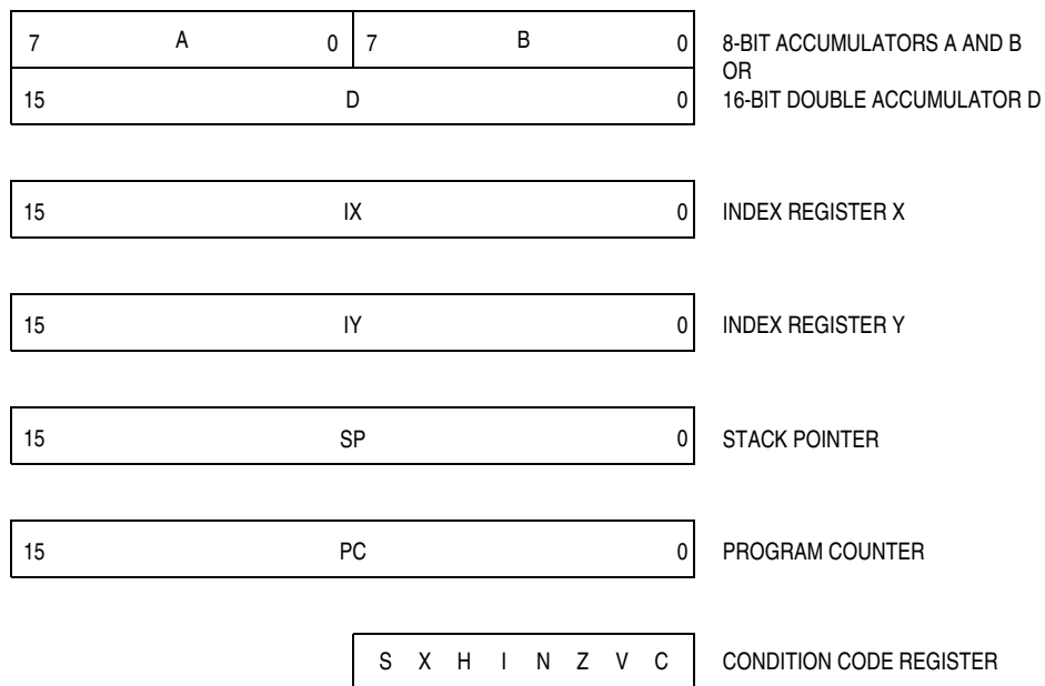
Figure 2-1. Programming Model
