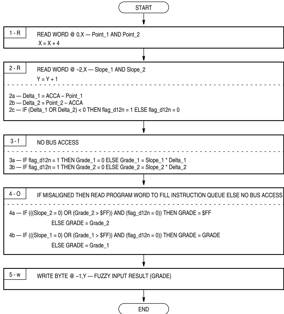
Figure 9-5. MEM Instruction Flow Diagram
