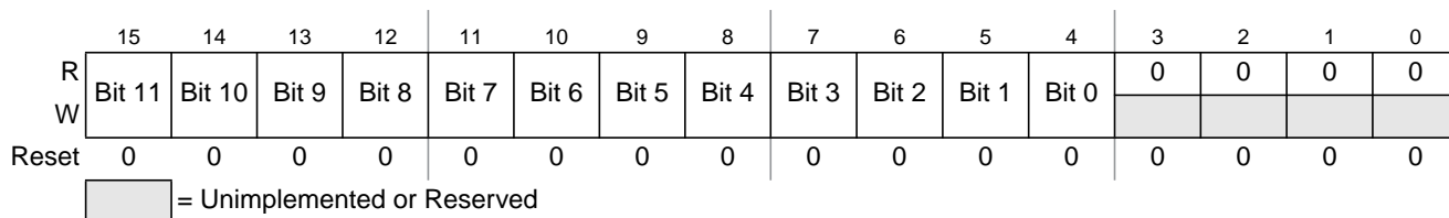
Figure 9-14. Left justified ATD conversion result register (ATDDR n )
