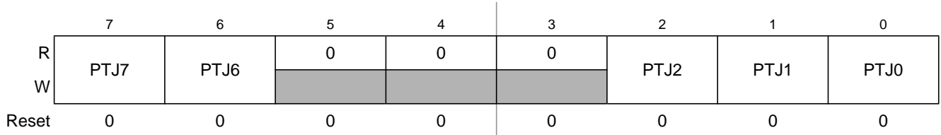
Figure 2-47. Port J Data Register (PTJ)
