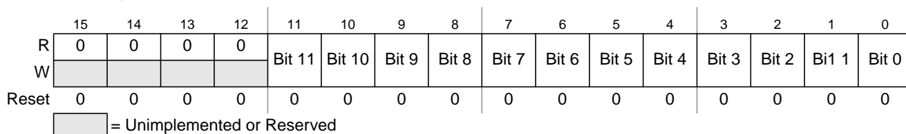
Figure 9-15. Right justified ATD conversion result register (ATDDR n )
