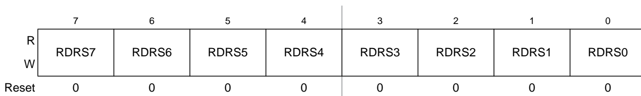
Figure 24-24. Port S Reduced Drive Register (RDRS)
