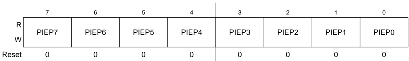
Figure 23-46. Port P Interrupt Enable Register (PIEP)
