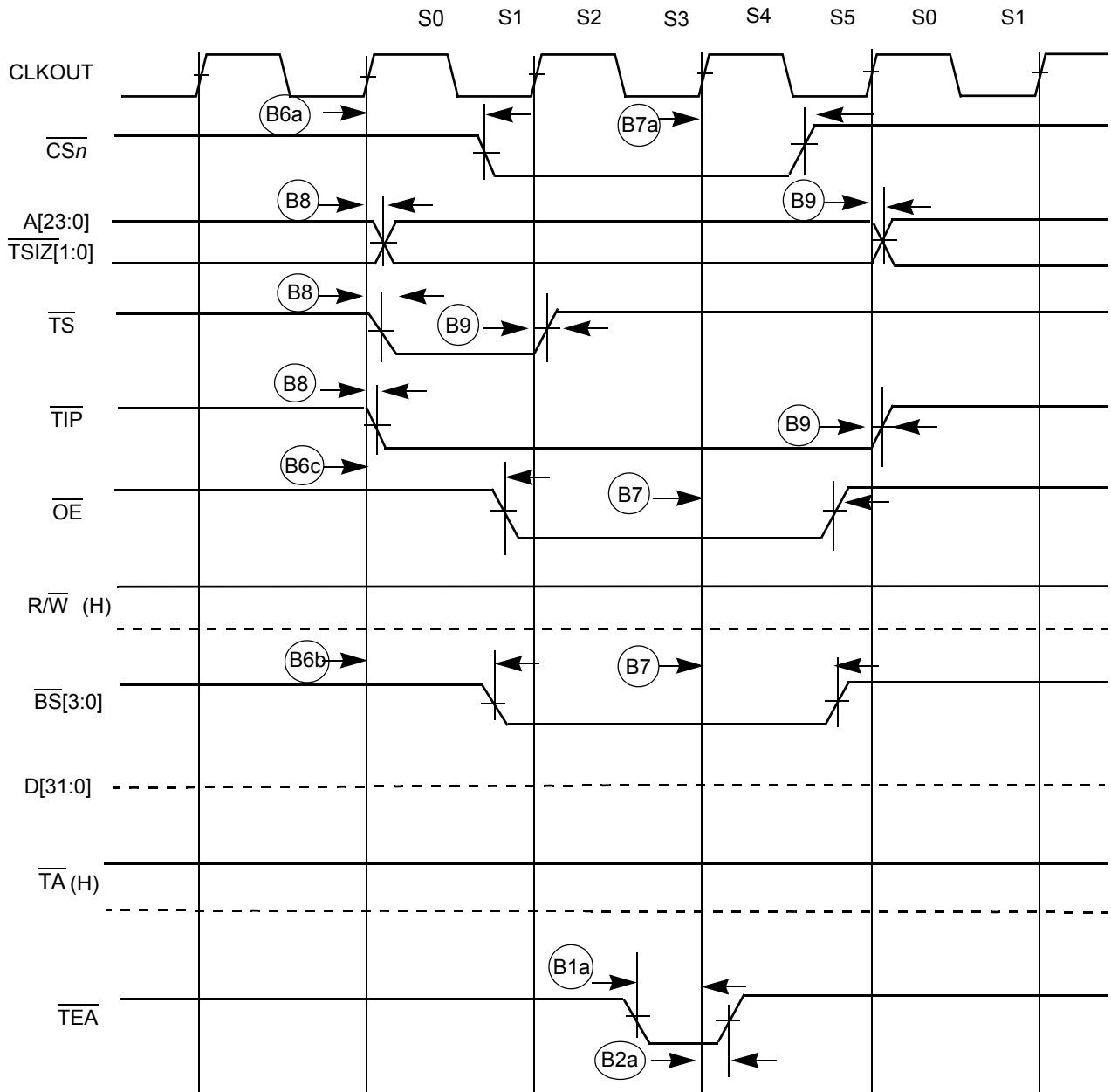
Figure 9. SRAM Read Bus Cycle Terminated by TEA
