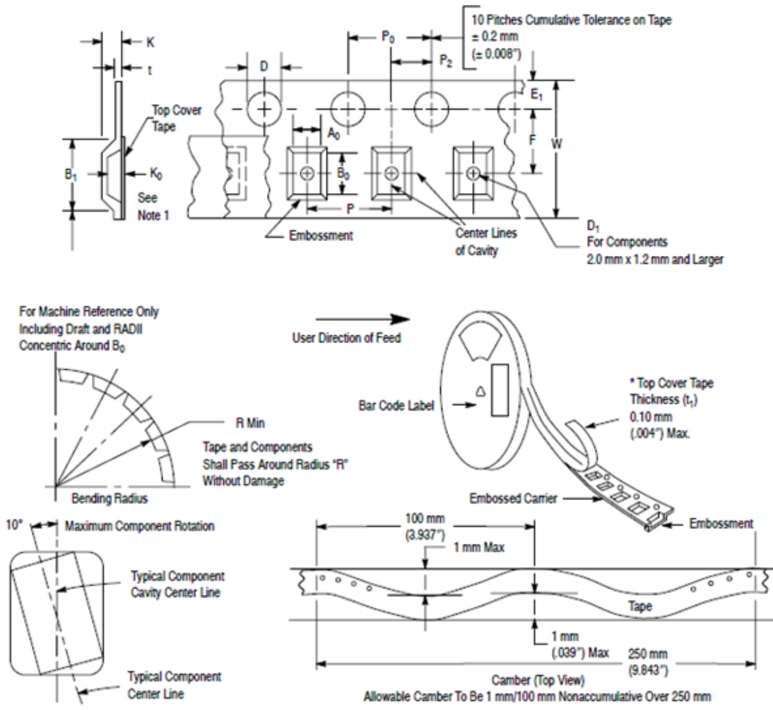
Figure 37. Tape-and-Reel Example
