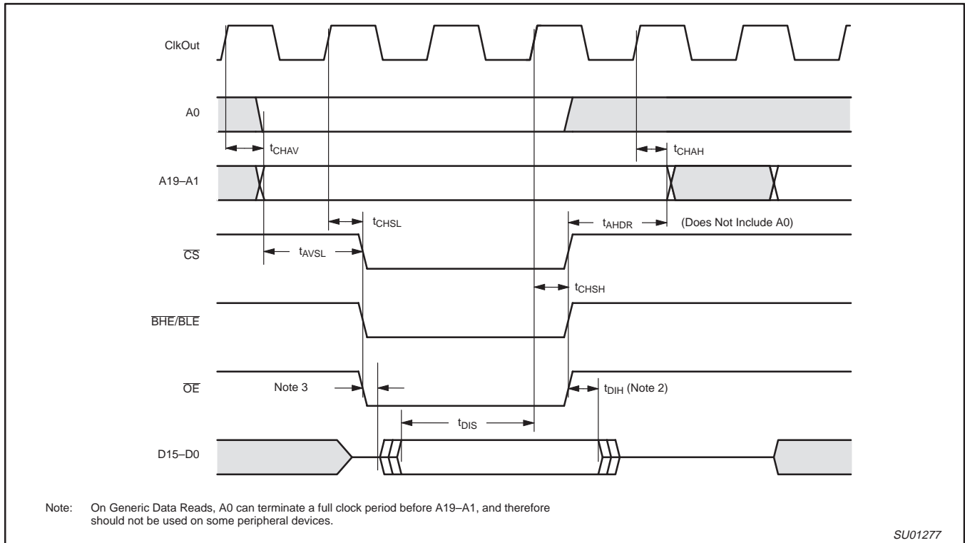
Figure 7. Generic (SRAM, ROM, Flash, I/O Devices, etc.) Read on 16-Bit Bus
