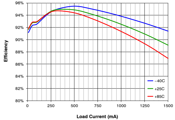
Figure 6. Efficiency vs. Load Current and Temperature, V_{IN} = 3.0\text{ V} , V_{OUT} = 3.5\text{ V}
