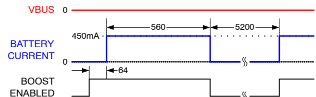
Figure 41. Boost Response Attempting to Start into V_{BUS} Short Circuit (times in \mu\text{s} )
