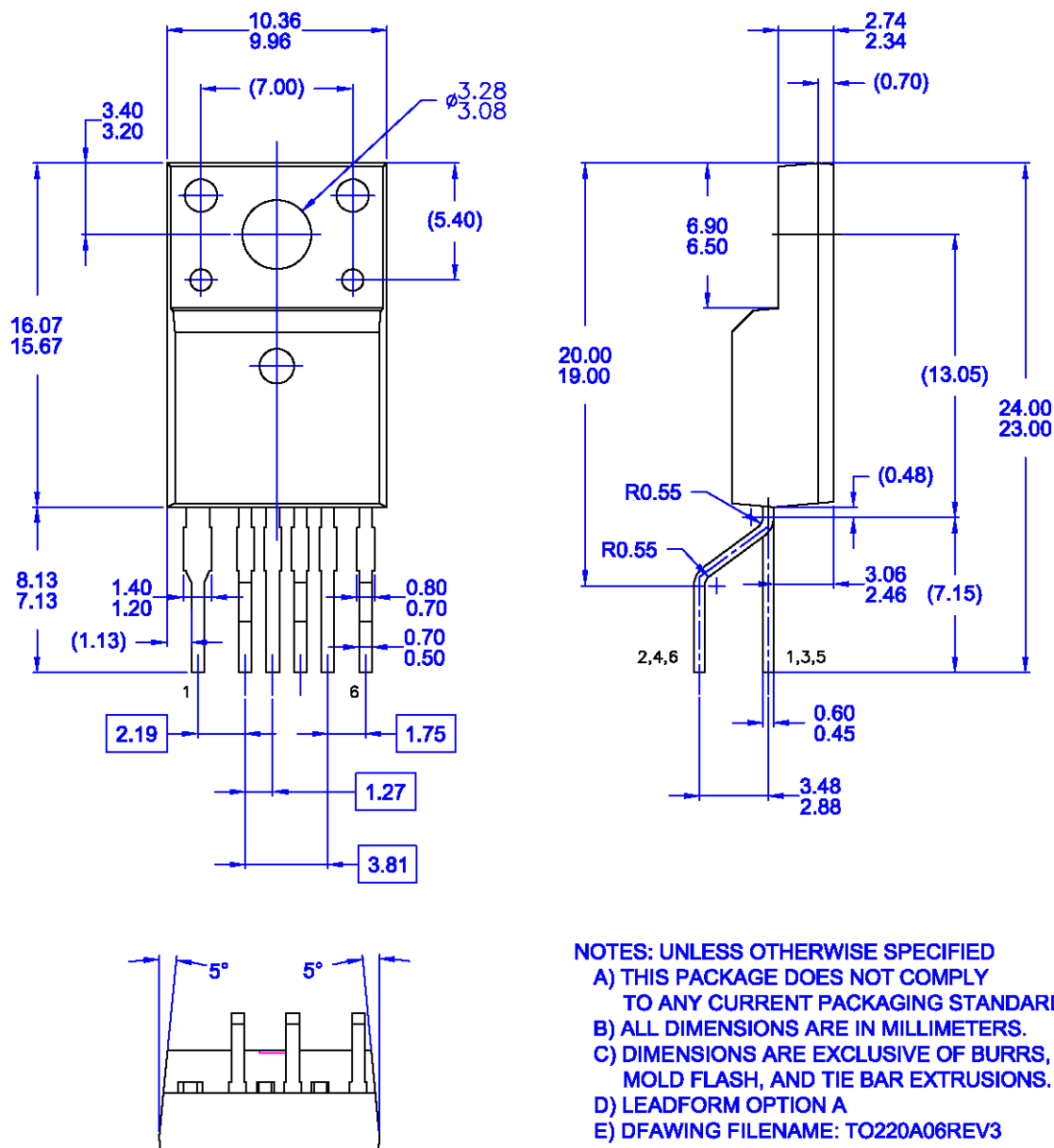
Figure 41. 6-Lead, TO-220 Package
