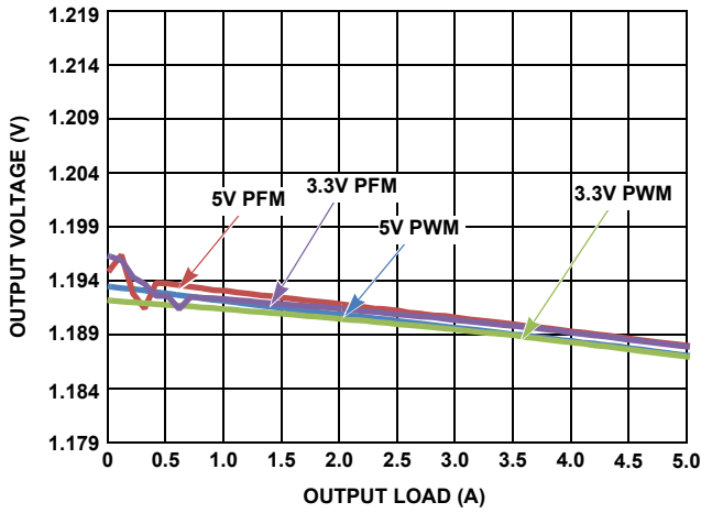
FIGURE 11. V_{\text{OUT}} REGULATION vs LOAD ( V_{\text{OUT}} = 1.2\text{V} )
