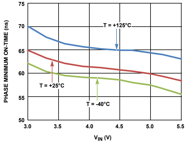
FIGURE 14. PHASE MINIMUM ON-TIME vs V_{\text{IN}}
