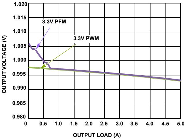
FIGURE 13. V_{\text{OUT}} REGULATION vs LOAD ( V_{\text{OUT}} = 1.0\text{V} )
