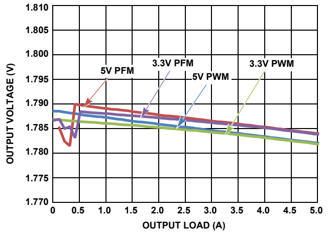
FIGURE 12. V_{\text{OUT}} REGULATION vs LOAD ( V_{\text{OUT}} = 1.8\text{V} )
