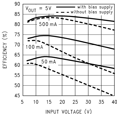
Figure 43. Effects of Bias Supply Feature on 5V Regulator Efficiency
