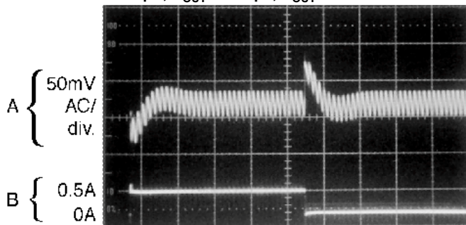
A: Output Voltage, 50 mV/div. (AC) B: 200 mA to 500 mA Load Pulse
