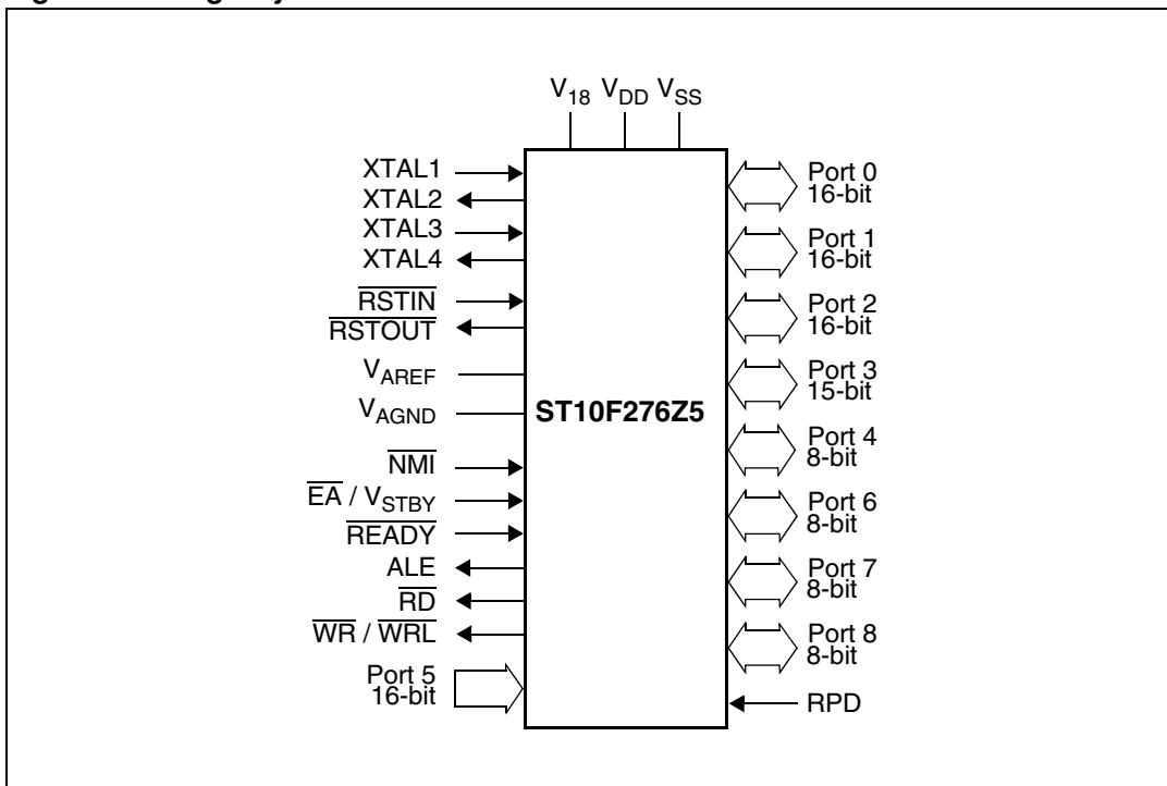
Figure 1. Logic symbol
