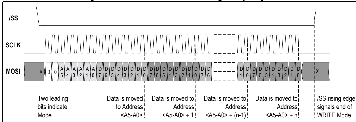
Figure 11. SPI communication: writing multiple bytes
