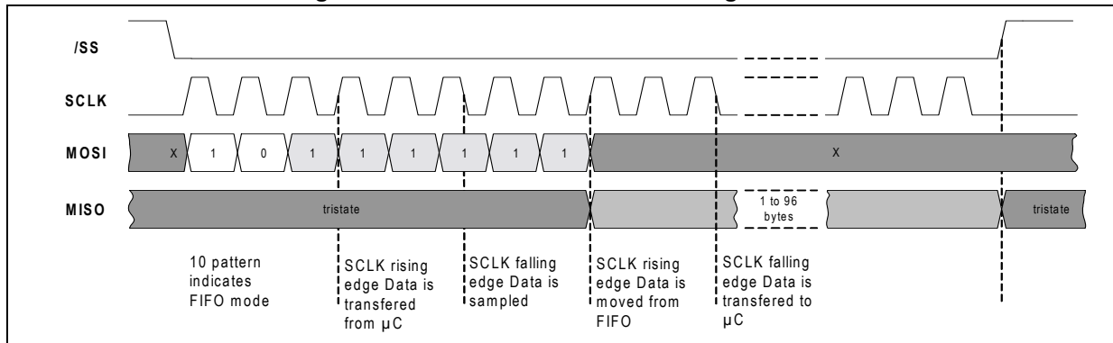
Figure 14. SPI communication: reading of FIFO
