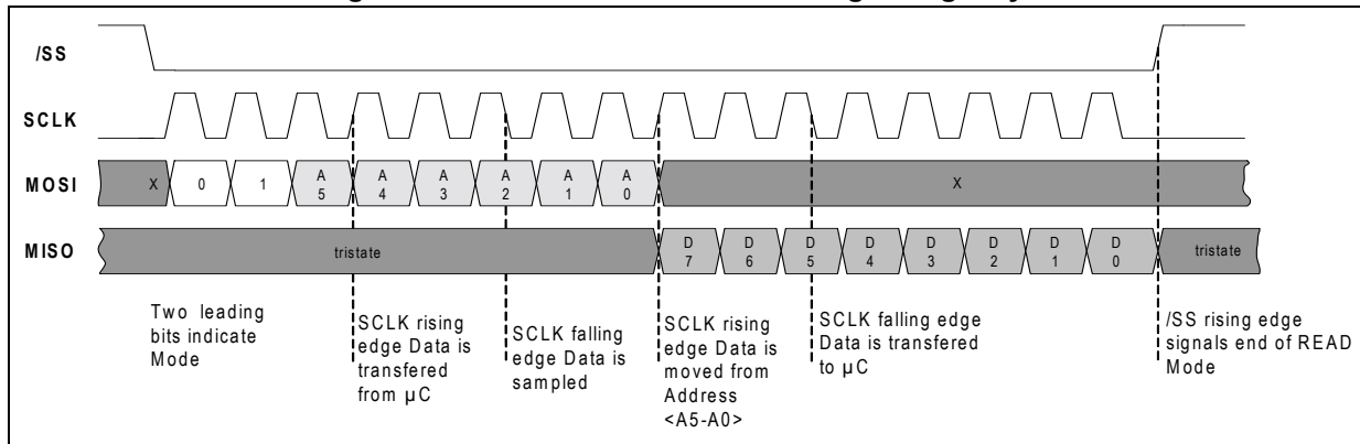
Figure 12. SPI communication: reading a single byte
