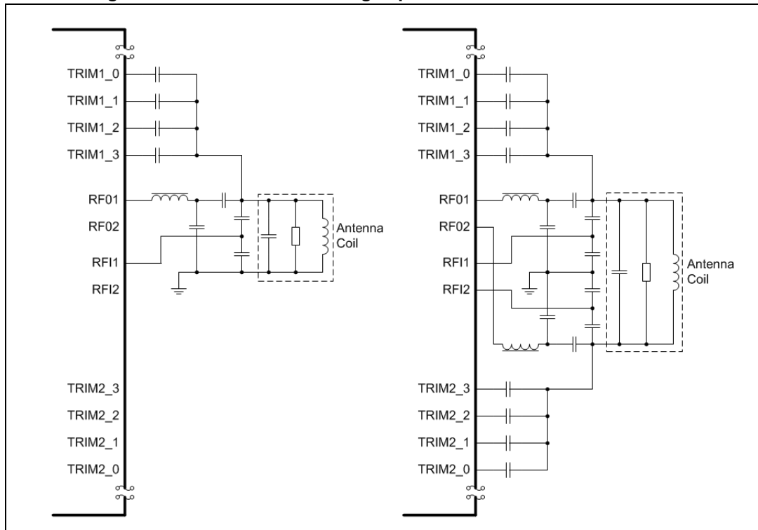
Figure 26. Connection of tuning capacitors to the antenna LC tank
