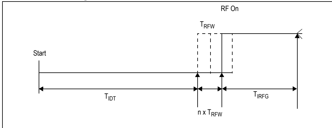
Figure 19. Direct command NFC Initial Field ON
