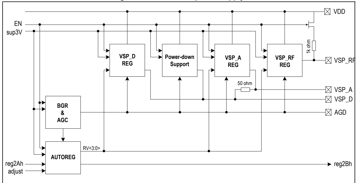
Figure 8. ST25R3911B power supply
