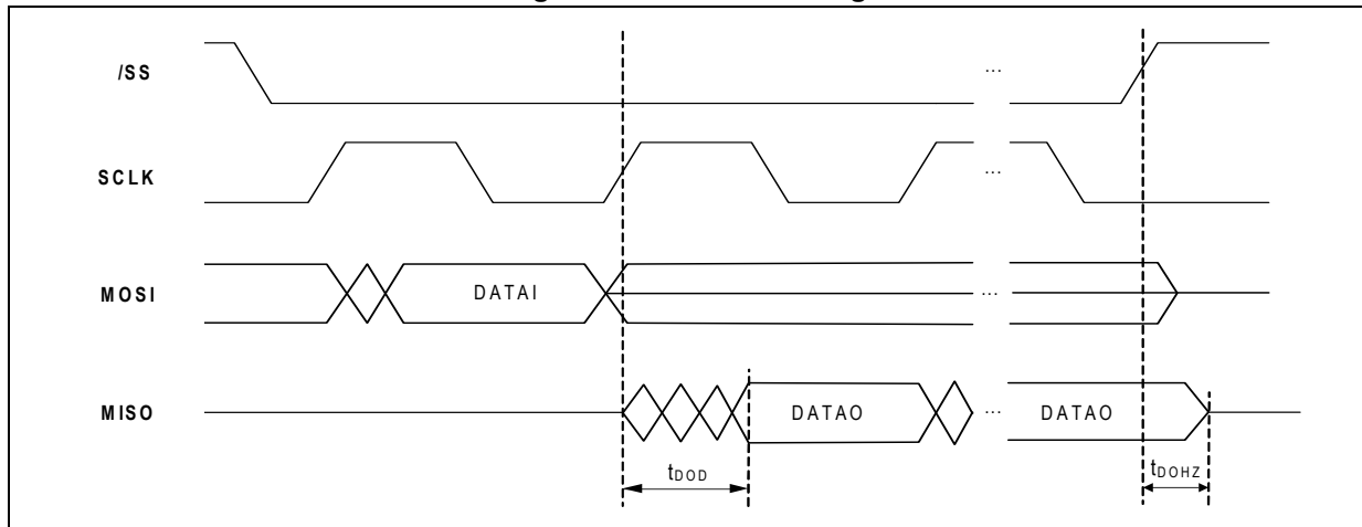
Figure 18. SPI read timing
