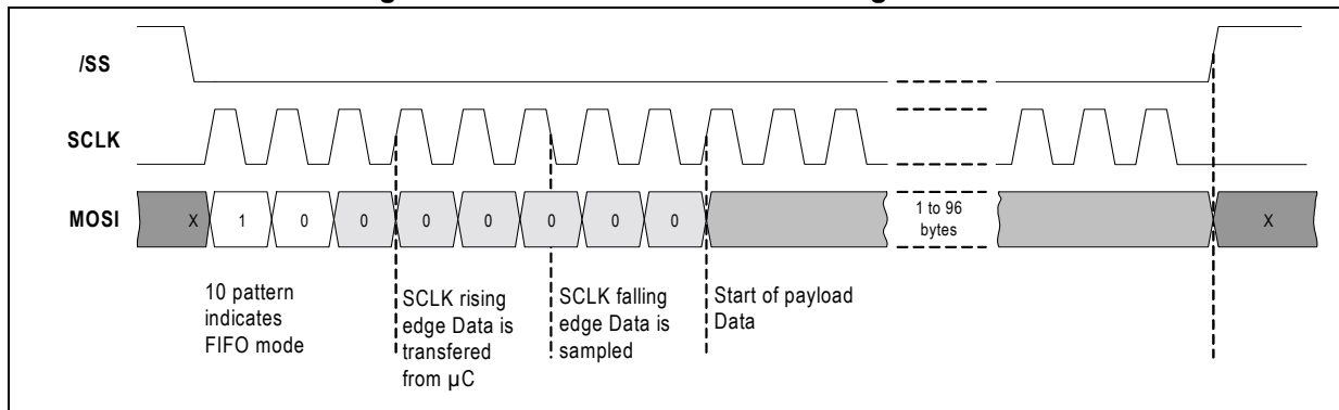
Figure 13. SPI communication: loading of FIFO
