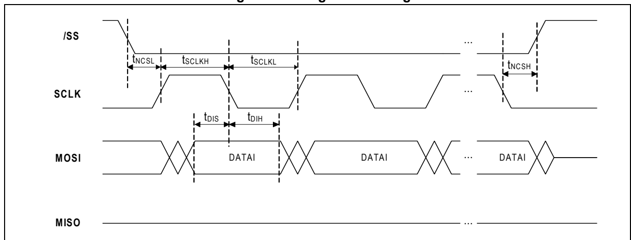
Figure 17. SPI general timing
