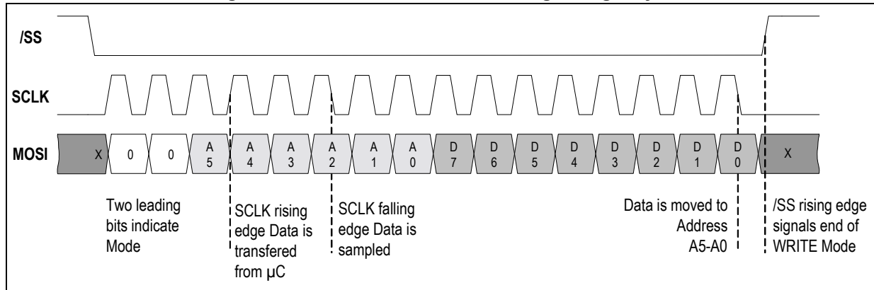
Figure 10. SPI communication: writing a single byte
