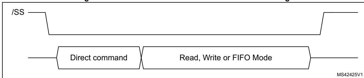
Figure 16. SPI communication: direct command chaining
