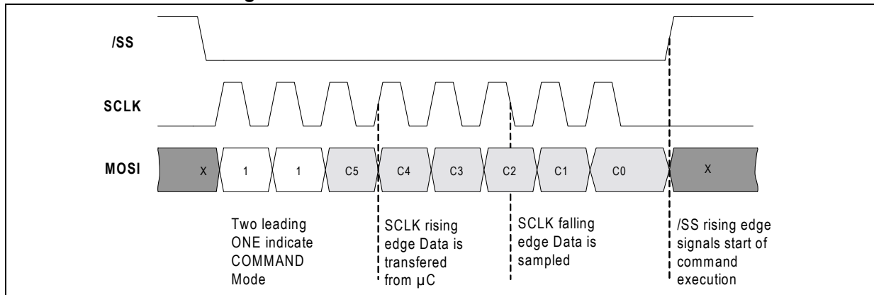
Figure 15. SPI communication: direct command
