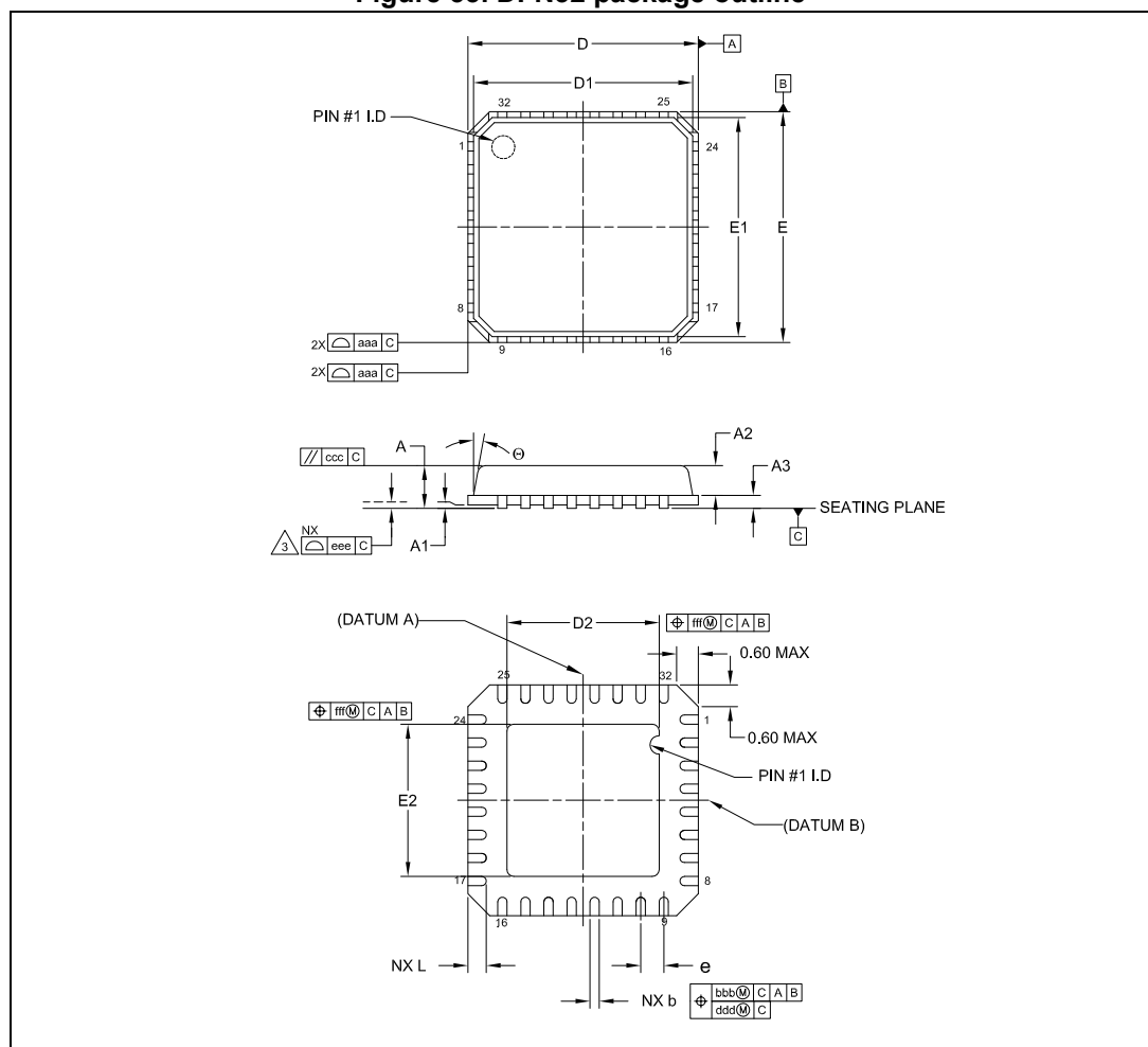
Figure 33. DFN32 package outline
