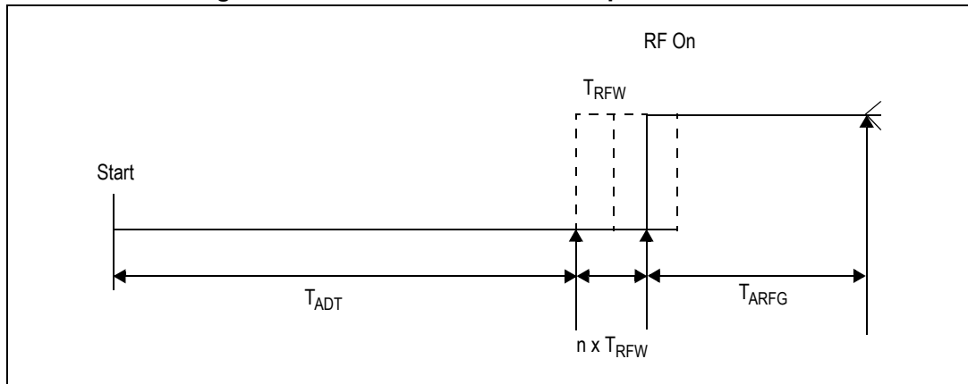
Figure 20. Direct command NFC Response Field ON
