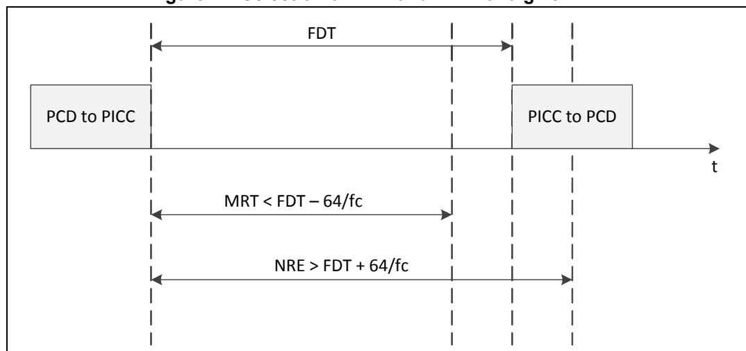
Figure 22. Selection of MRT and NRT for a given FDT
