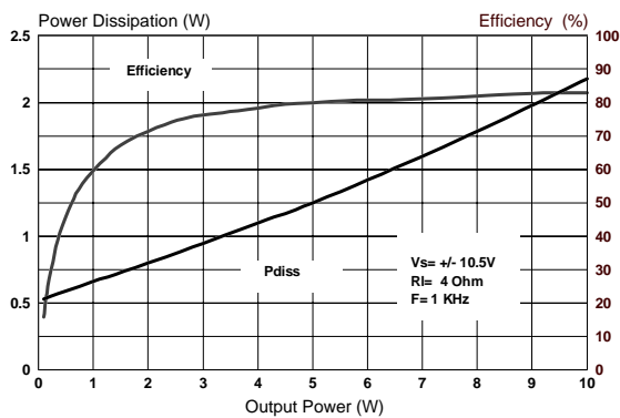
Figure 9. Power Dissipation and Efficiency vs. Output Power
