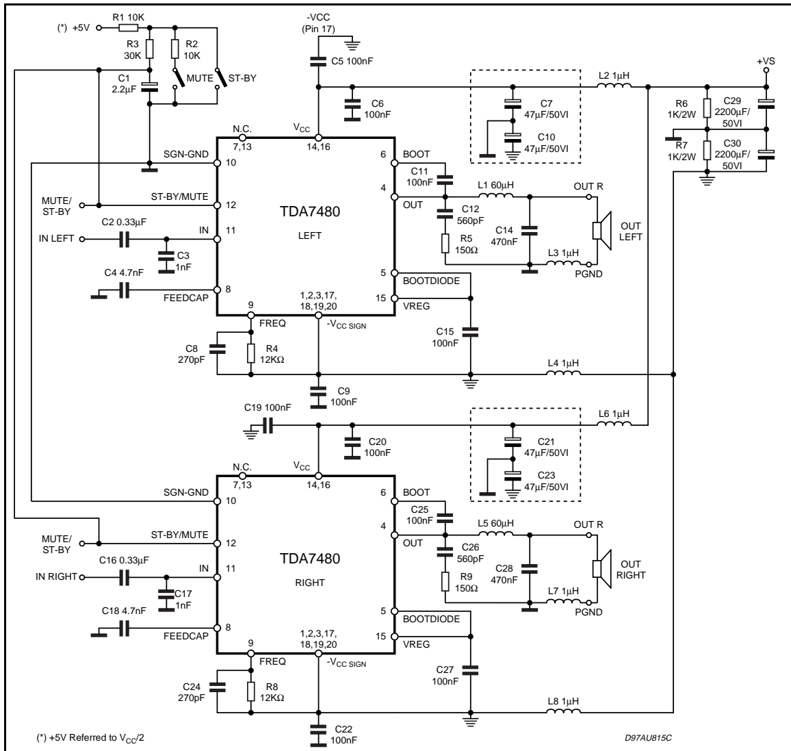
Figure 3: Stereo Application in Single Supply.
