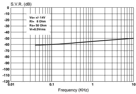
Figure 11. Supply Voltage Rejection vs. Frequency
