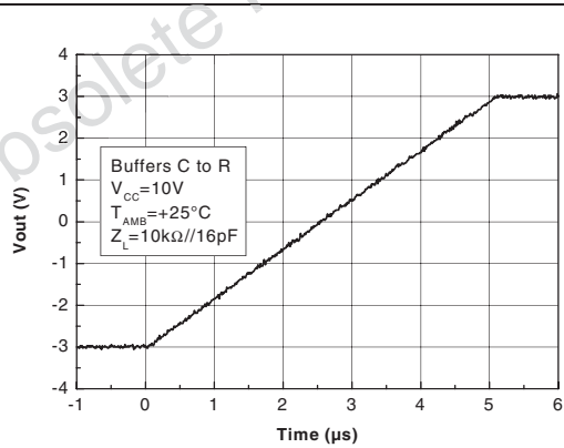
Figure 29. Large signal response - buffers C to R
