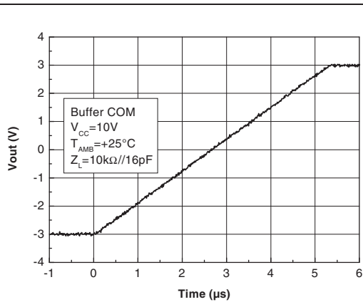
Figure 31. Large signal response - buffer COM
