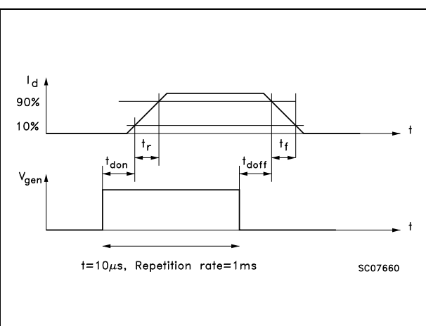
Figure 29. Waveforms
