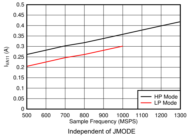
图 7-106. Single Channel, I_{VA11} vs FS
