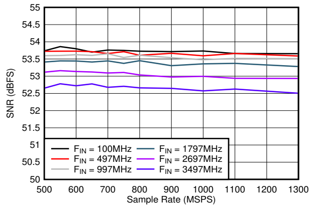
图 7-22. SNR vs Sample Rate
