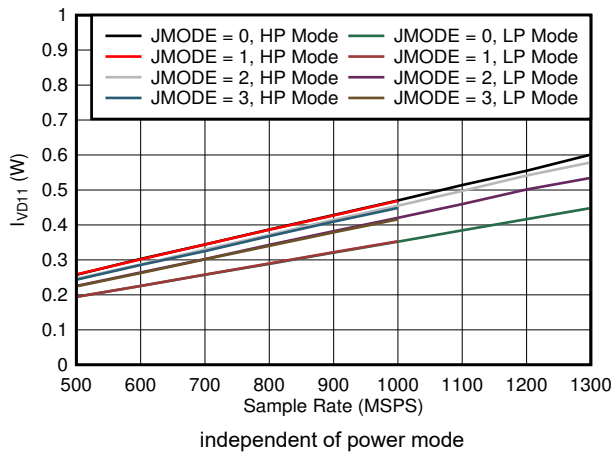
图 7-87. Quad Channel, I_{VD11} vs FS and JMODE 0 - 3
