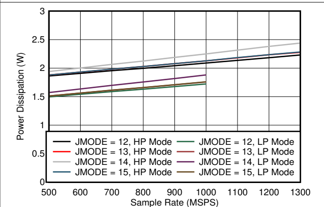
图 7-84. Quad Channel, Power Dissipation vs FS for JMODES 12 - 15
