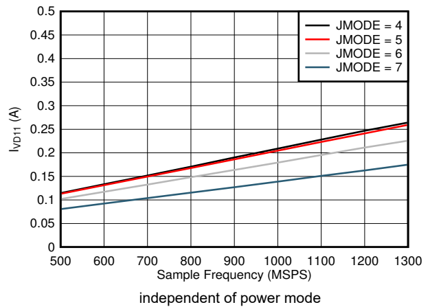
图 7-108. Single Channel, I_{VD11} vs FS and JMODE 4 - 7
