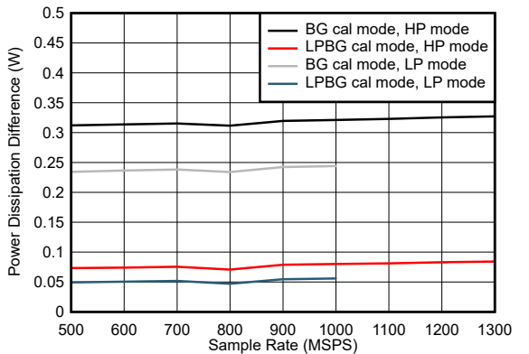
图 7-111. Quad Channel, Power Dissipation Change with Calibration Mode
