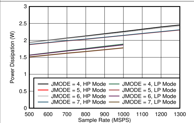
图 7-82. Quad Channel, Power Dissipation vs FS for JMODES 4 - 7
