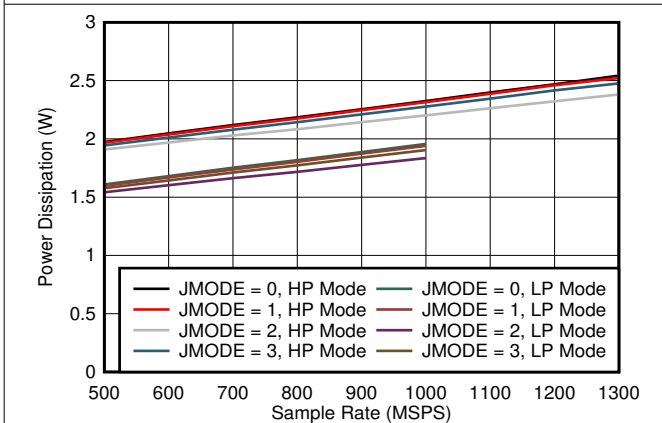
图 7-81. Quad Channel, Power Dissipation vs FS for JMODES 0 - 3
