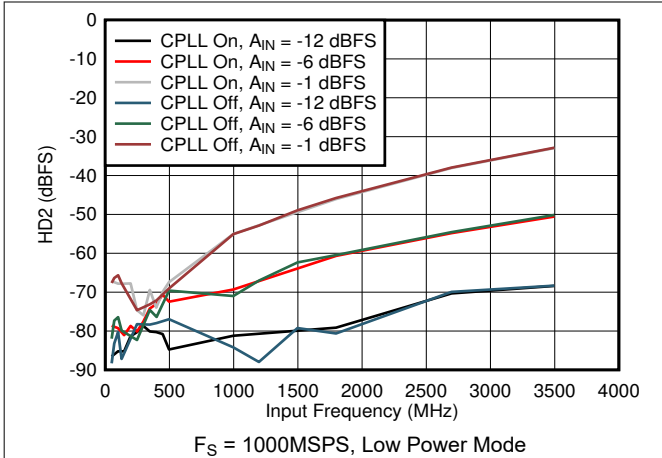
图 7-79. HD2 vs Input Frequency, CPLL and Input Amplitude
