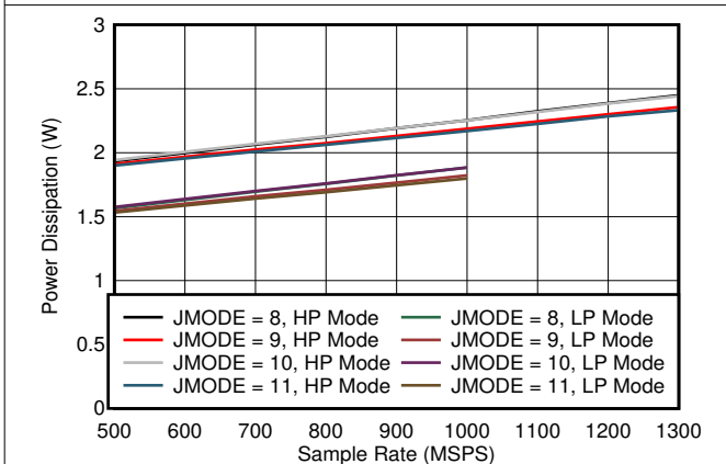
图 7-83. Quad Channel, Power Dissipation vs FS for JMODES 8 - 11
