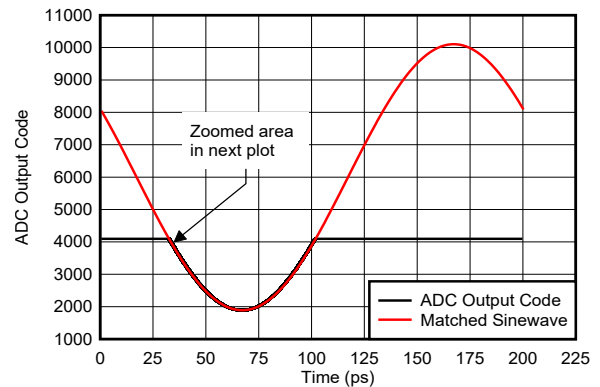
图 6-148. Sinewave Overdrive Recovery
