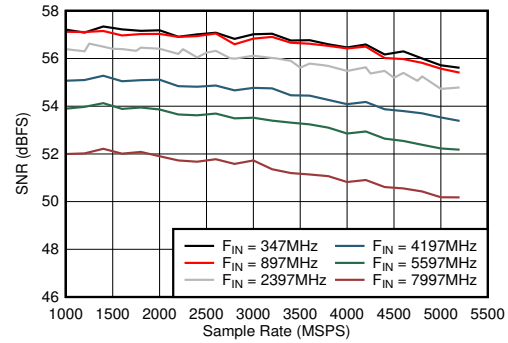
图 6-44. Dual Channel Mode: SNR vs Sample Rate and Input Frequency A_{IN} = -1\text{ dBFS}
