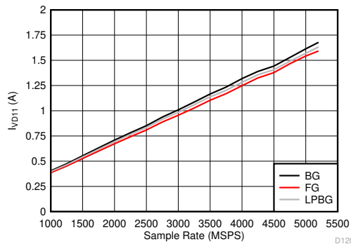
图 6-134. Dual Channel Mode: I_{VD11} vs Sample Rate
