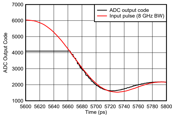
图 6-147. Pulse Overdrive Recovery Zoomed
