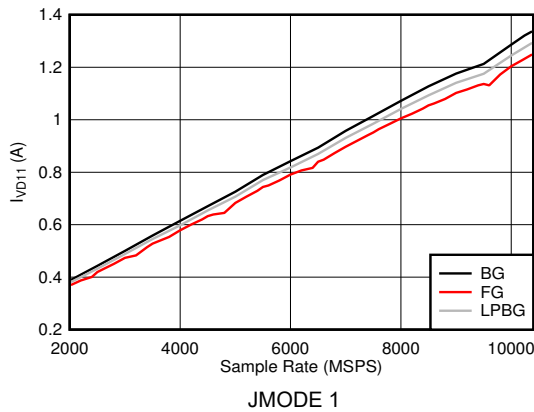
图 6-123. DES Mode: I_{VD11} vs Sample Rate
