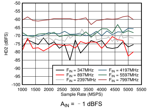
图 6-50. Dual Channel Mode: HD2 vs Sample Rate and Input Frequency
