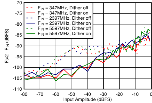
图 6-80. Dual Channel Mode: F_s/2 - F_{IN} vs Input Amplitude and Dither
