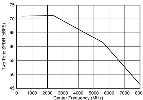
图 6-107. Dual Channel Mode: Two Tone SFDR vs Input Frequency
