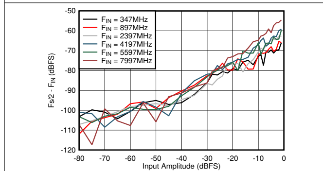
图 6-65. DES Mode: F_s/2 - F_{\text{IN}} vs Input Amplitude and Frequency
