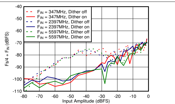
图 6-66. DES Mode: F_s/4 + F_{\text{IN}} vs Input Amplitude and Dither
