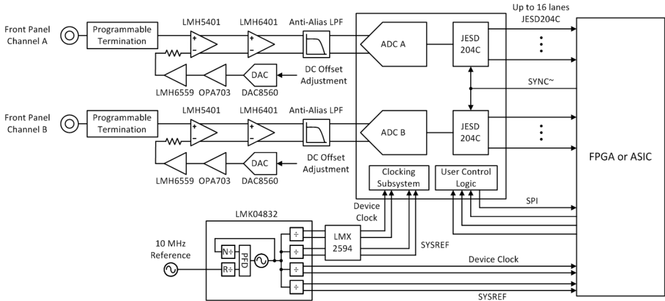
图 8-5. Typical Configuration for Reconfigurable Oscilloscope
