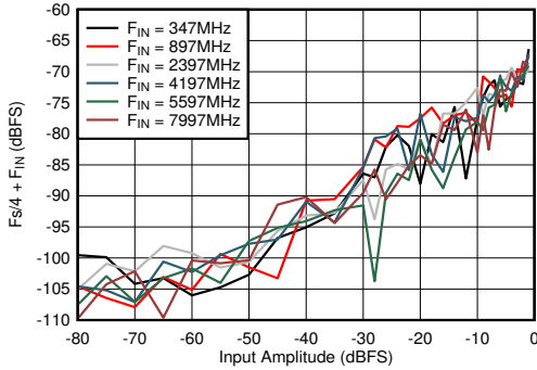
图 6-67. DES Mode: F_s/4 + F_{IN} vs Input Amplitude and Frequency
