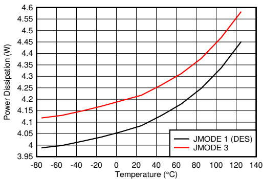
图 6-141. Power Dissipation vs Temperature
