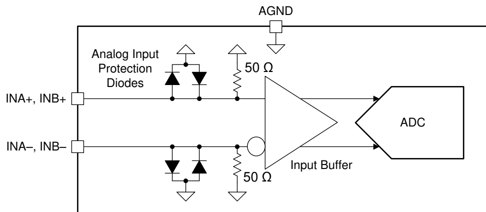
图 7-1. ADC12DJ5200RF Analog Input Internal Termination and Protection Diagram
