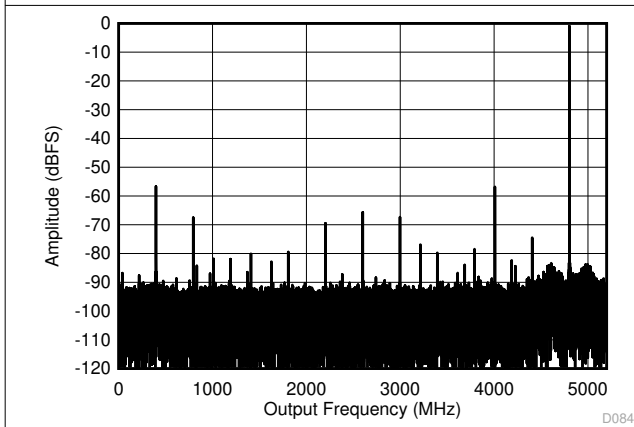
图 6-9. DES Mode: Single Tone FFT at 5597 MHz
