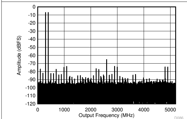
图 6-9. DES Mode: Single Tone FFT at 5597 MHz
