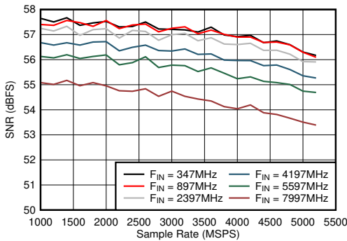
图 6-45. Dual Channel Mode: SNR vs Sample Rate and Input Frequency A_{IN} = -6\text{ dBFS}
