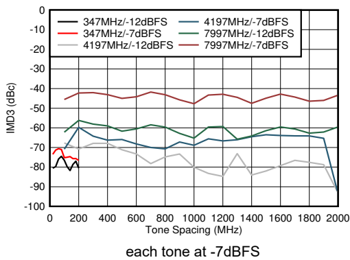
图 6-101. DES Mode: IMD3 vs Tone Spacing
