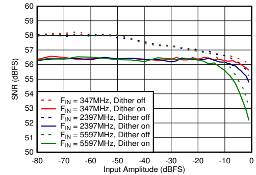
图 6-72. Dual Channel Mode: SNR vs Input Amplitude and Dither
