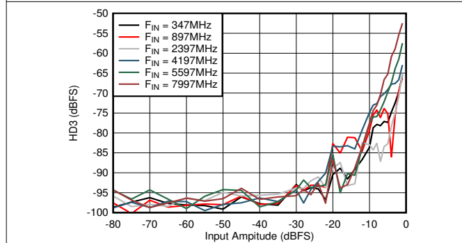
图 6-63. DES Mode: HD3 vs Input Amplitude and Frequency
