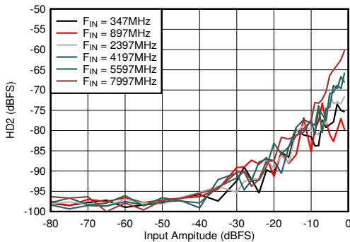
图 6-75. Dual Channel Mode: HD2 vs Input Amplitude and Frequency
