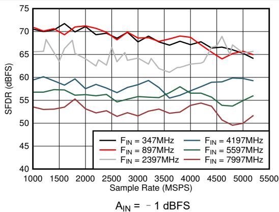
图 6-47. Dual Channel Mode: SFDR vs Sample Rate and Input Frequency A_{IN} = -1\text{ dBFS}
