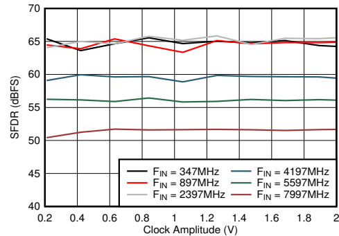
图 6-84. Dual Channel Mode: SFDR vs Clock Amplitude
