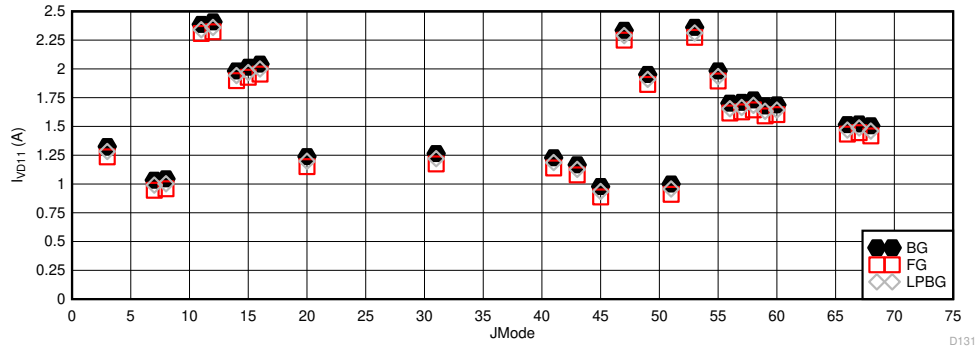
图 6-115. Dual Channel Mode: I_{VD11} vs JMODE at 5.2GSPS
