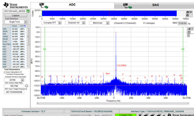
图 8-4. FFT for 497.77-MHz Input Signal, 2.7 GSPS, Decimation-by-16, f_{NCO} = 500 MHz, JMODE16
