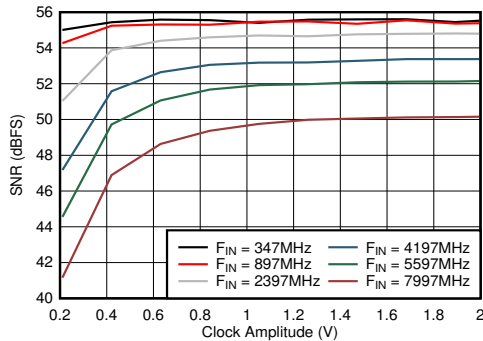
图 6-83. Dual Channel Mode: SNR vs Clock Amplitude
