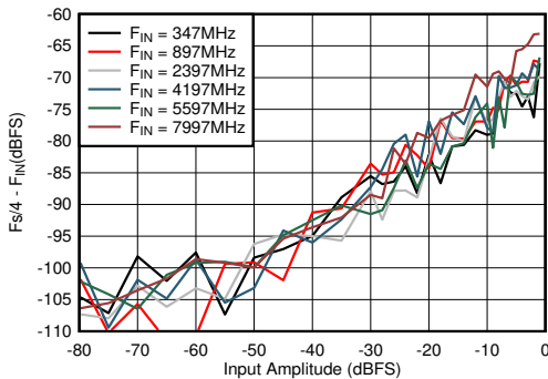
图 6-69. DES Mode: F_s/4 - F_{IN} vs Input Amplitude and Frequency
