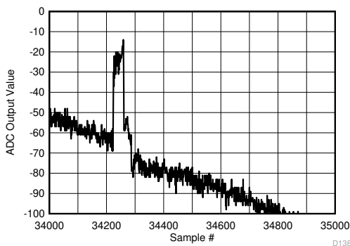
图 6-143. Background Calibration Core Transition (AC Signal - zoomed)
