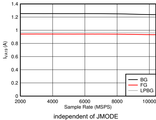
图 6-121. DES Mode: I_{VA19} vs Sample Rate
