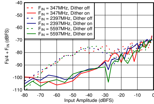
图 6-68. DES Mode: F_s/4 + F_{IN} vs Input Amplitude and Dither
