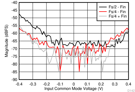
图 6-98. F_s/2 - F_{IN} and F_s/4 \pm F_{IN} vs Input Common Mode Voltage
