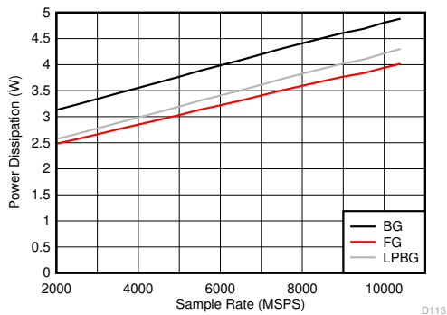
图 6-127. DES Mode: Power Dissipation vs Sample Rate
