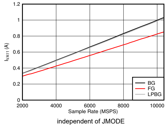
图 6-122. DES Mode: I_{VA11} vs Sample Rate
