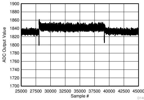
图 6-145. Background Calibration Core Transition (DC Signal - zoomed)
