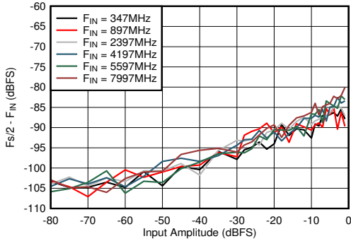
图 6-79. Dual Channel Mode: F_s/2 - F_{IN} vs Input Amplitude and Frequency
