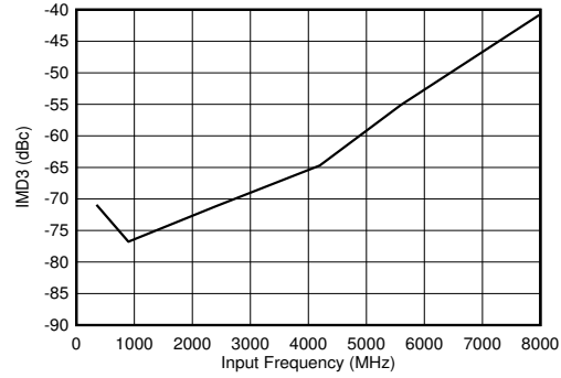
图 6-104. Dual Channel Mode: IMD3 vs Input Frequency each tone at -7dBFS
