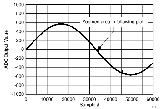
图 6-142. Background Calibration Core Transition (AC Signal)
