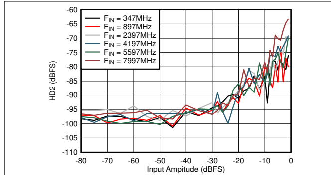
图 6-61. DES Mode: HD2 vs Input Amplitude and Frequency
