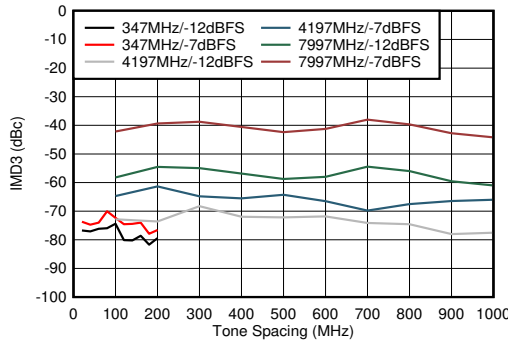
图 6-106. Dual Channel Mode: IMD3 vs Tone Spacing
