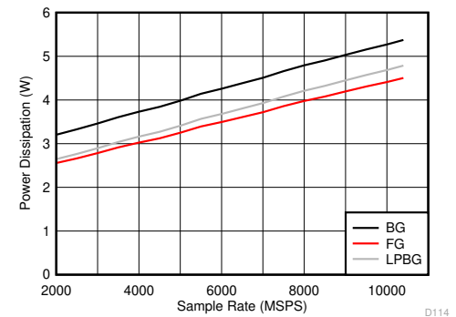
图 6-128. DES Mode: Power Dissipation vs Sample Rate
