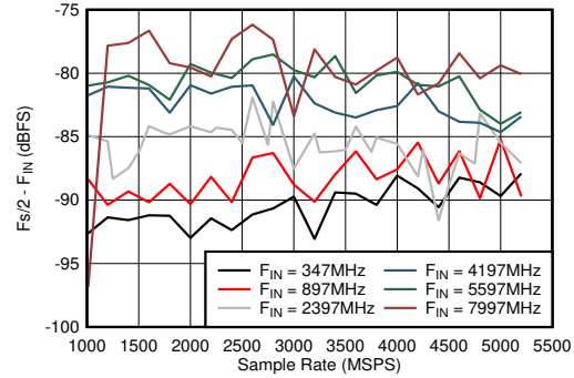
图 6-56. Dual Channel Mode: F_s/2 - F_{IN} vs Sample Rate and Input Frequency
