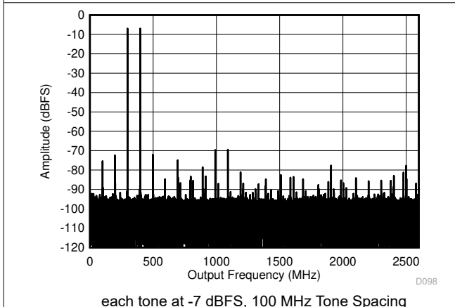
图 6-23. Dual Channel Mode: Two Tone FFT at 347 MHz
