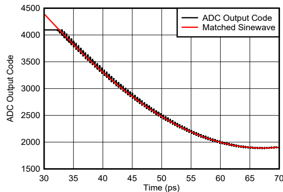
图 6-149. Sinewave Overdrive Recovery
