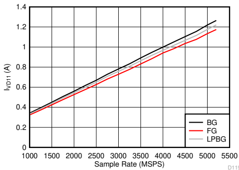
图 6-133. Dual Channel Mode: I_{VD11} vs Sample Rate
