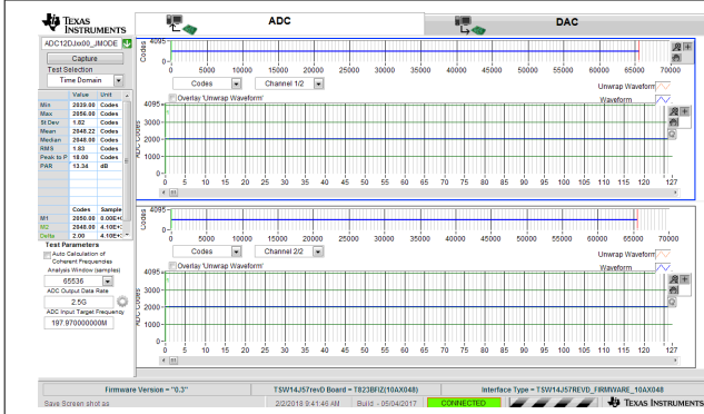
图 8-10. Idle-Channel Noise (No Input) for 2.5-GSPS, Dual-Channel Oscilloscope
