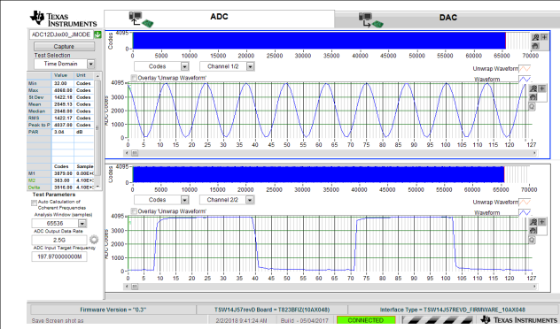
图 8-11. 200-MHz, Sine-Wave (Channel A) and 40-MHz, Square-Wave (Channel B) Time Domain for 5-GSPS, Single-Channel Oscilloscope
