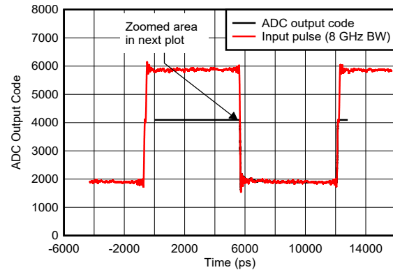
图 6-146. Pulse Overdrive Recovery
