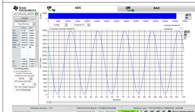
图 8-8. 200-MHz, Sine-Wave Time Domain for 5-GSPS, Single-Channel Oscilloscope
