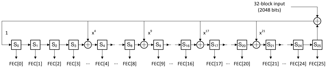
图 7-22. FEC Parity Bit Generator
