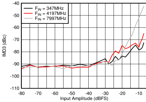
图 6-105. Dual Channel Mode: IMD3 vs Input Amplitude
