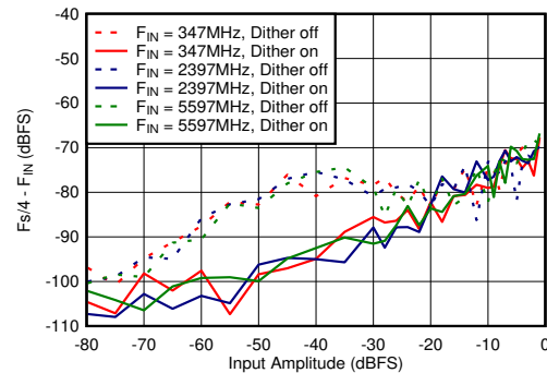
图 6-70. DES Mode: F_s/4 - F_{IN} vs Input Amplitude and Dither
