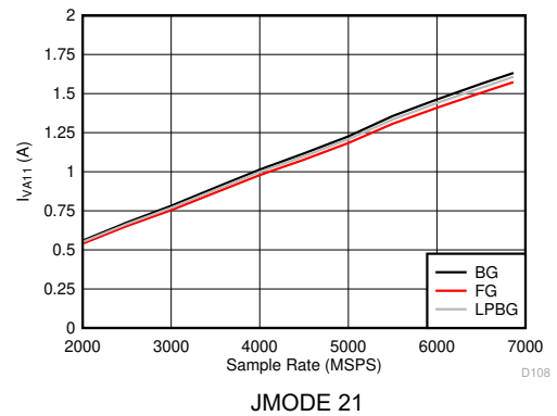
图 6-124. DES Mode: I_{VD11} vs Sample Rate
