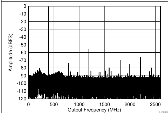
图 6-21. Dual Channel Mode: Single Tone FFT at 5597 MHz
