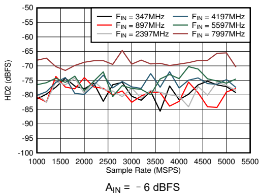
图 6-51. Dual Channel Mode: HD2 vs Sample Rate and Input Frequency
