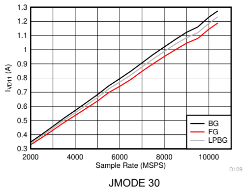
图 6-125. DES Mode: I_{VD11} vs Sample Rate
