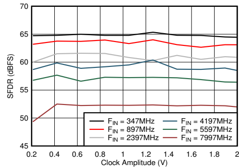
图 6-82. DES Mode: SFDR vs Clock Amplitude
