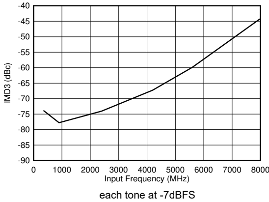
图 6-99. DES Mode: IMD3 vs Input Frequency
