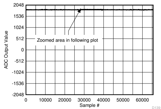
图 6-144. Background Calibration Core Transition (DC Signal)
