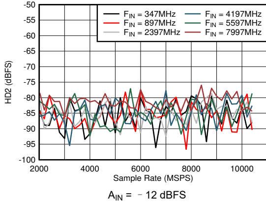
图 6-37. DES Mode: HD2 vs Sample Rate and Input Frequency
