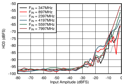
图 6-77. Dual Channel Mode: HD3 vs Input Amplitude and Frequency
