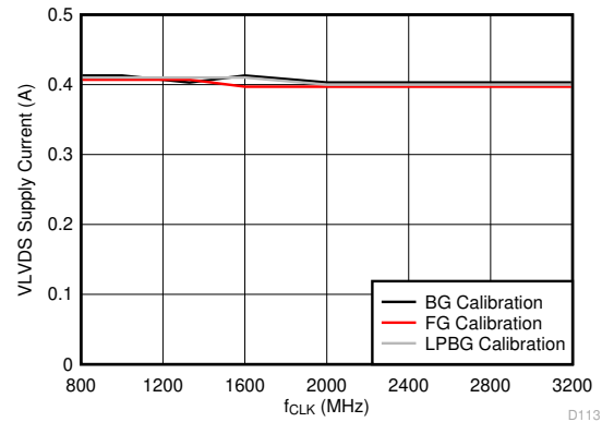
图 6-69. VLVD5 Supply Current vs Clock Rate
