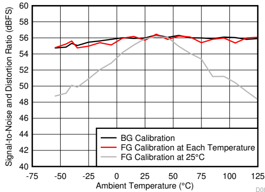
图 6-58. SINAD vs Temperature and Calibration Mode
