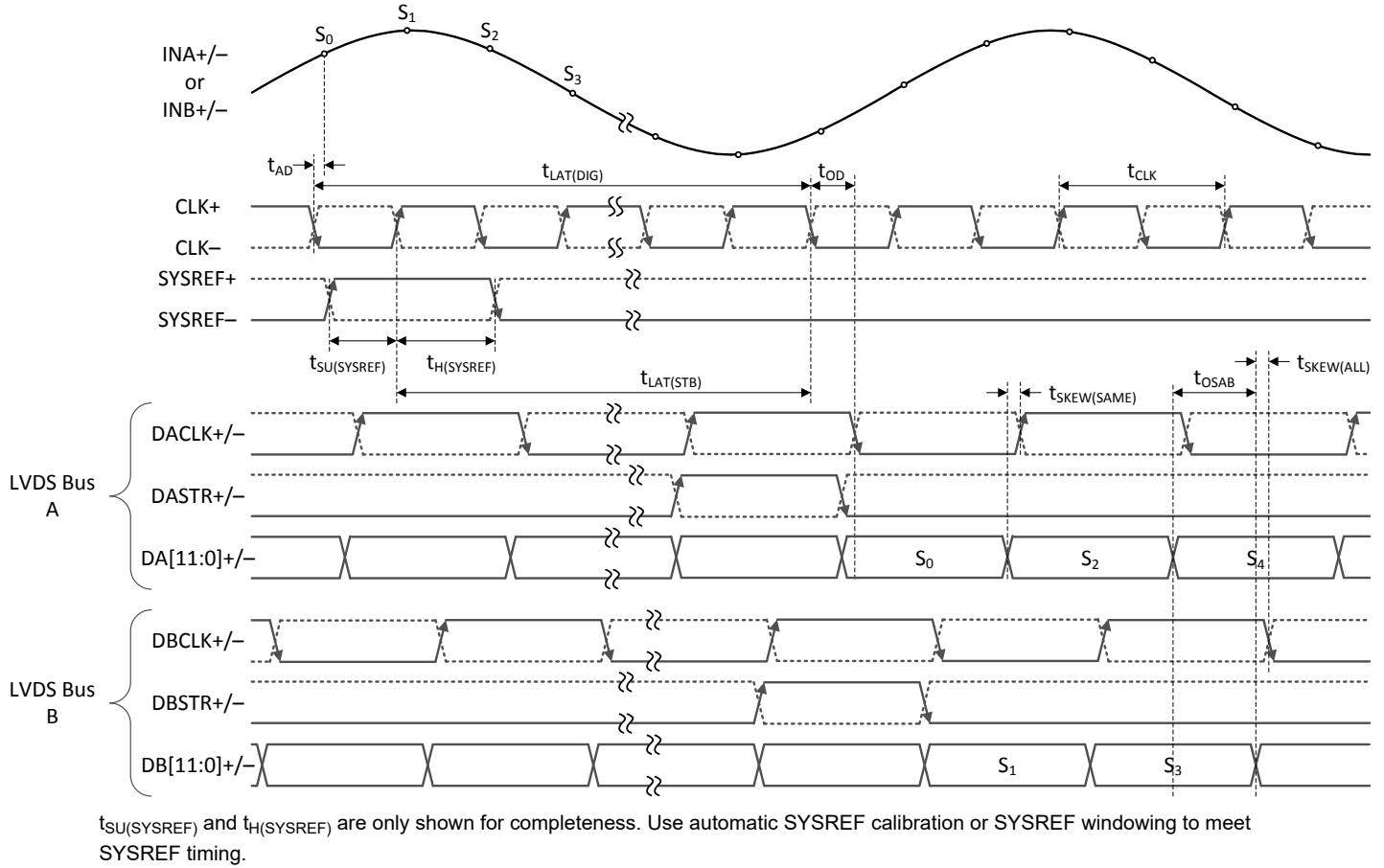
图 6-4. Single-Channel, 2-Bus, Staggered-Mode Timing (LDEMUX = 0, DES_EN = 1, LALIGNED = 0)
