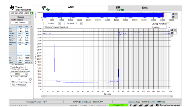
图 8-6. 40-MHz, Square-Wave Time Domain for 5-GSPS, Single-Channel Oscilloscope
