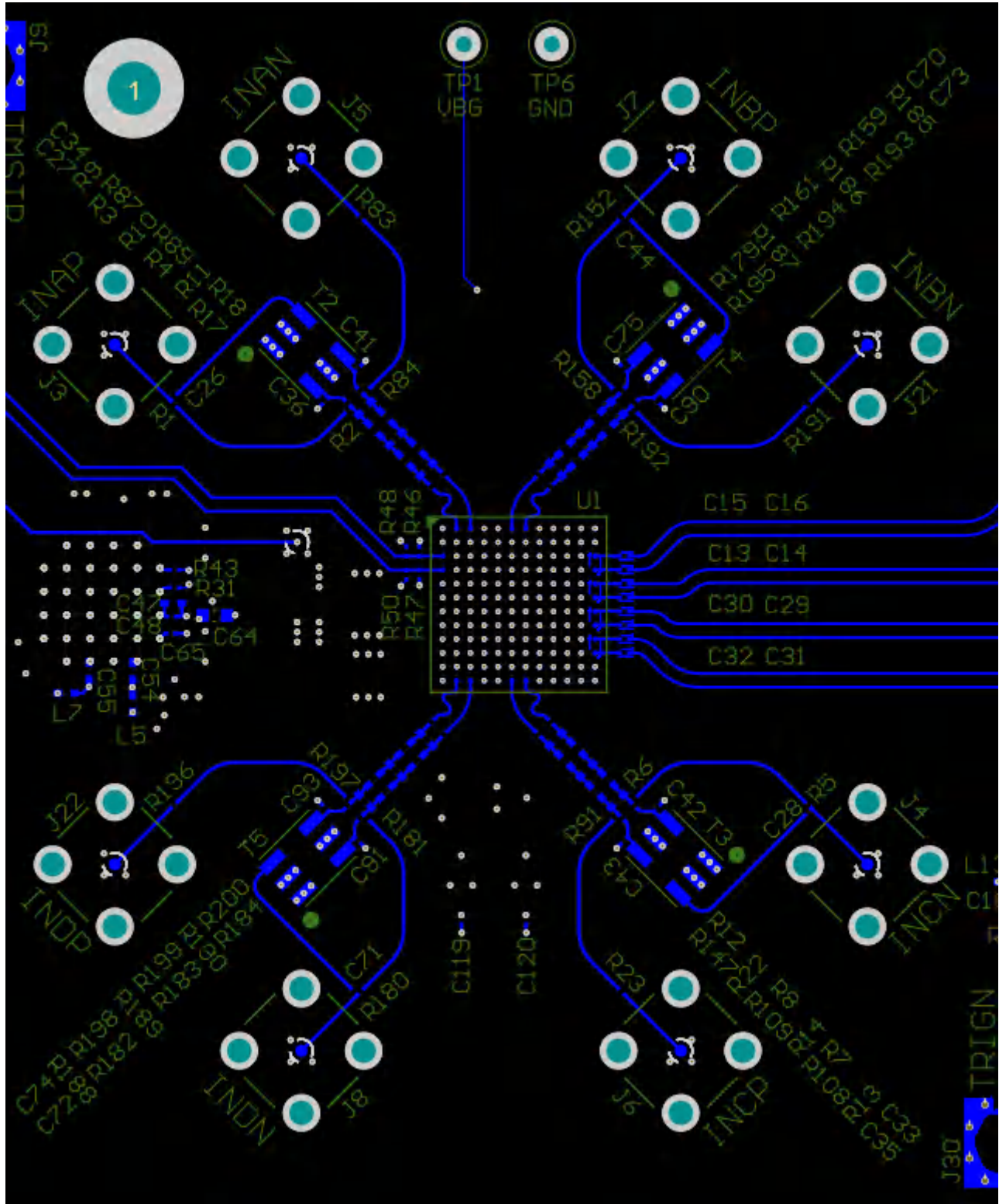
图 12-1. Top Layer Routing: Analog Inputs (INA±, INB±, INC±, IND±), TMSTP± and D[3:0]± Routing
