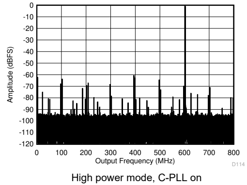
图 8-8. Single Tone FFT at 997 MHz and -1 dBFS
