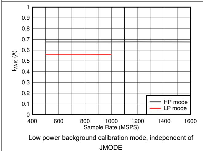
图 8-83. Quad Channel, I_{VA19} vs F_S
