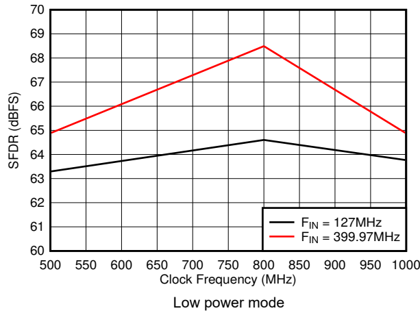
图 8-27. SFDR vs Sample Rate
