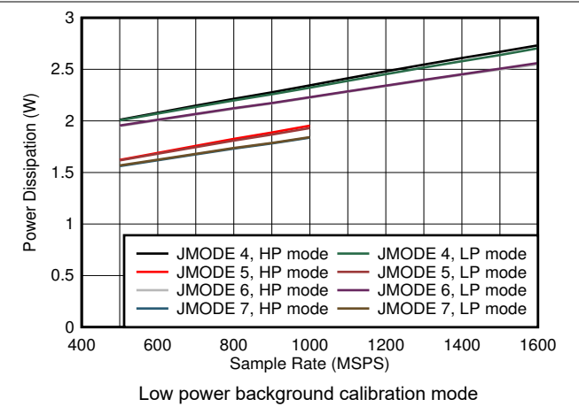
图 8-80. Quad Channel, Power Dissipation vs F_S and JMODE 4 - 7
