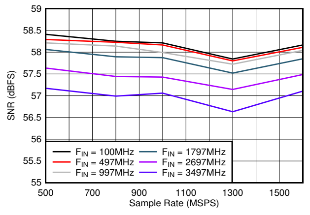
图 8-24. SNR vs Sample Rate
