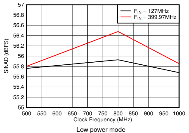
图 8-30. SINAD vs Sample Rate
