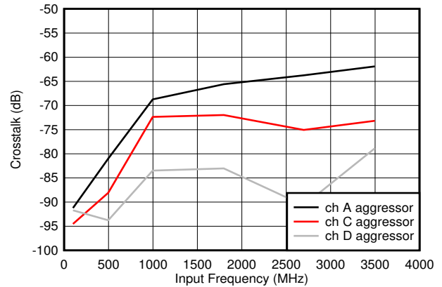
图 8-78. Crosstalk to Channel B vs F_{IN}
