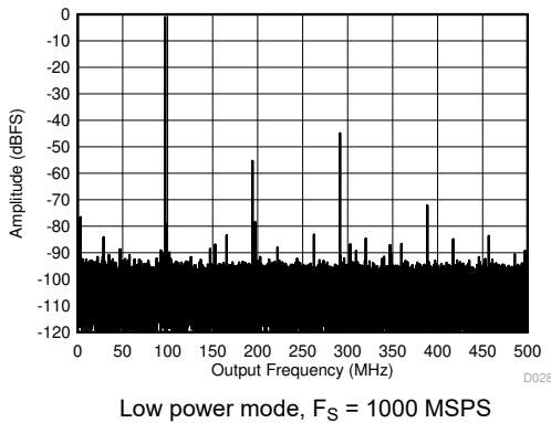
图 8-15. Single Tone FFT at 2097 MHz and -1 dBFS
