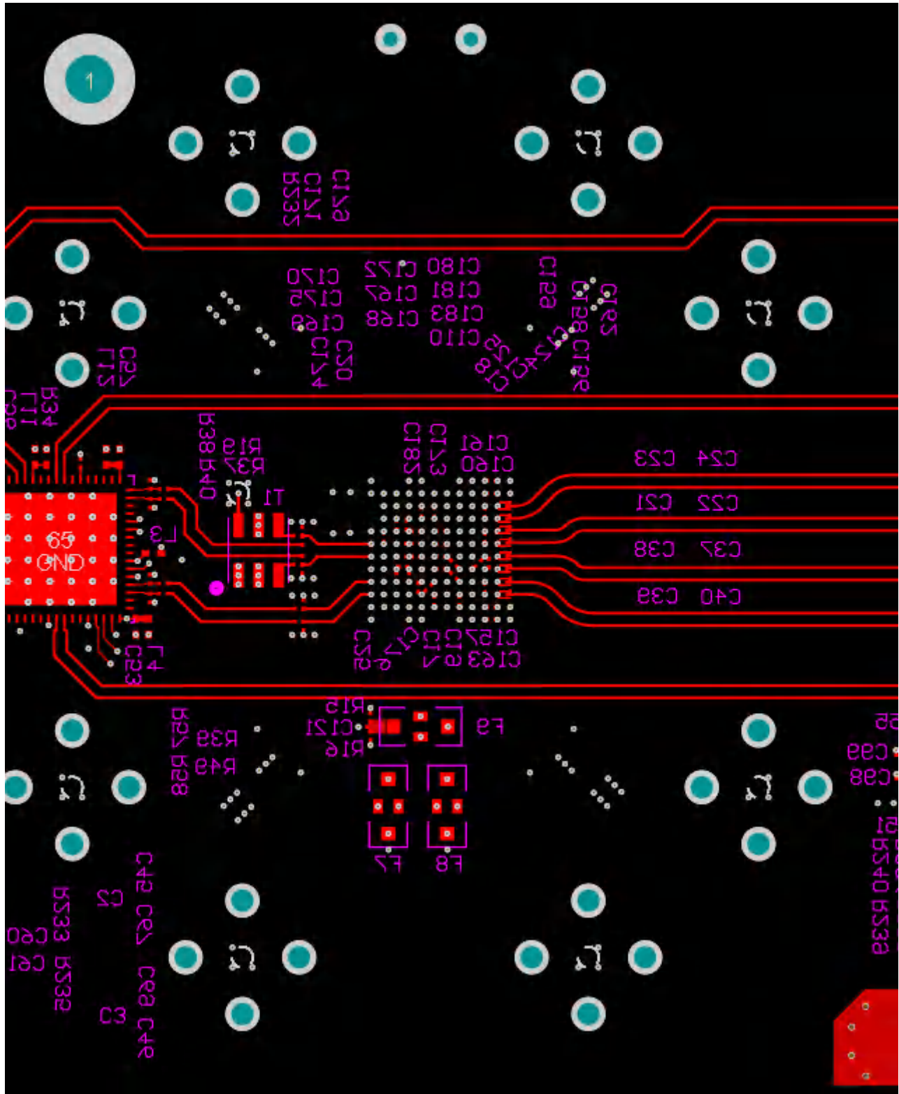
图 12-3. Bottom Layer Routing: CLK±, SYSREF and D[7:4]± Routing
