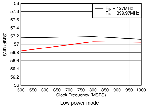
图 8-28. SNR vs Sample Rate
