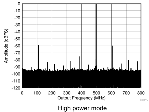
图 8-10. Single Tone FFT at 1797 MHz and -1 dBFS
