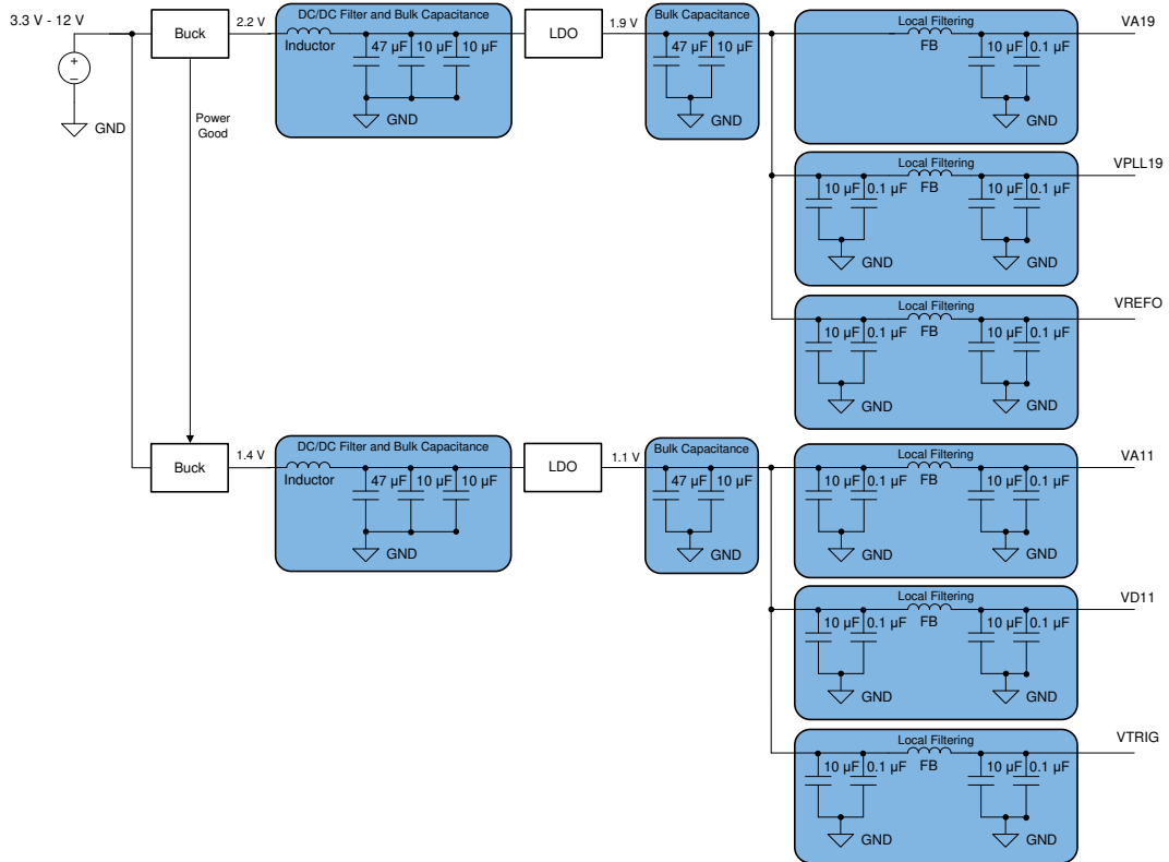
图 11-1. LDO Linear Regulator Approach Example
