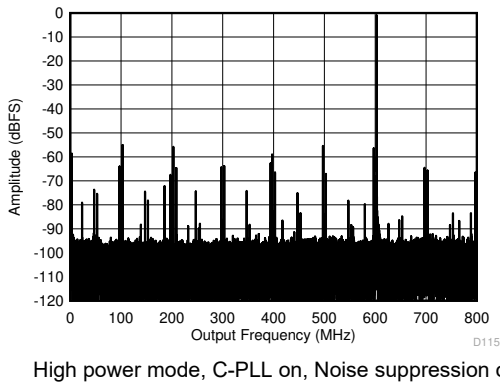
图 8-9. Single Tone FFT at 997 MHz and -1 dBFS
