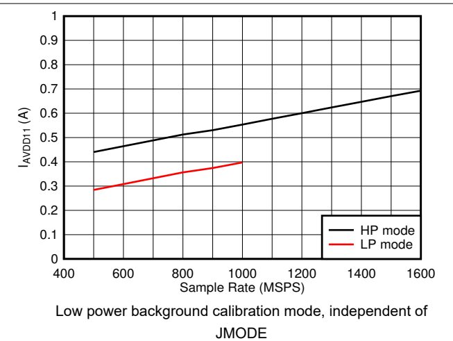
图 8-84. Quad Channel, I_{VA11} vs F_S
