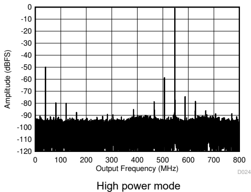
图 8-11. Single Tone FFT at 3797 MHz and -1 dBFS
