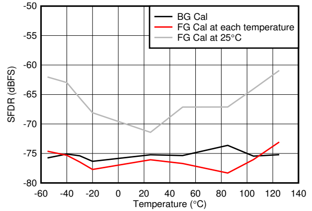
图 8-68. Worst Spur vs Temperature
