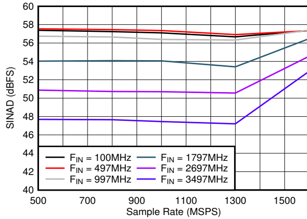
图 8-25. SINAD vs Sample Rate
