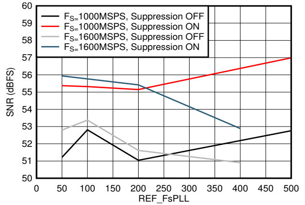
图 8-38. SNR vs F_{REF} and Suppression
