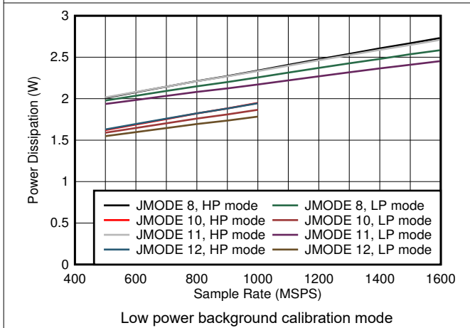
图 8-81. Quad Channel, Power Dissipation vs F_S and JMODE 8 - 12
