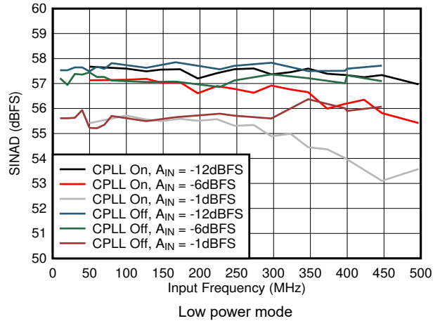
图 8-56. SINAD vs A_{IN} and C-PLL
