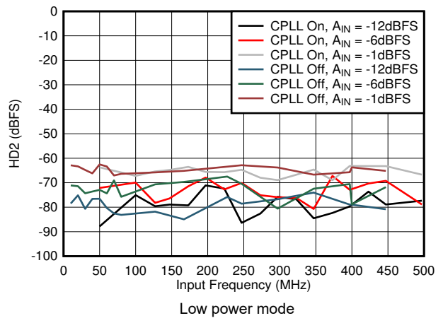
图 8-58. HD2 vs A_{IN} and C-PLL
