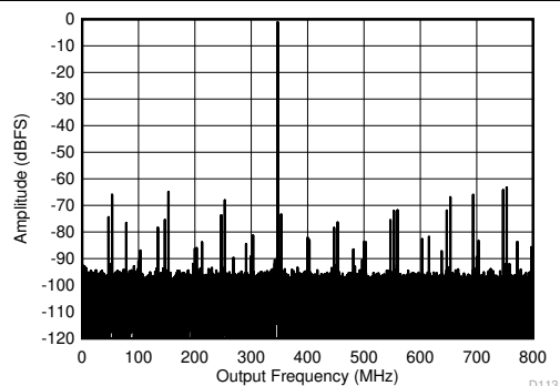
图 8-6. Single Tone FFT at 347 MHz and -1 dBFS
