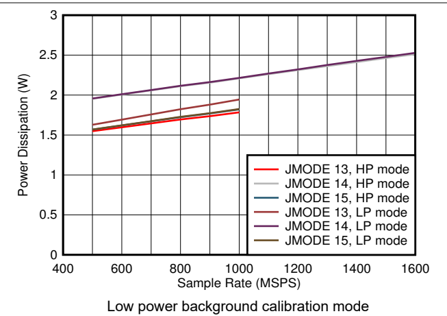
图 8-82. Quad Channel, Power Dissipation vs F_S and JMODE 13 - 15
