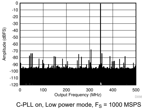
图 8-13. Single Tone FFT at 347 MHz and -1 dBFS
