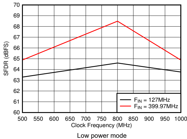
图 8-29. SFDR vs Sample Rate
