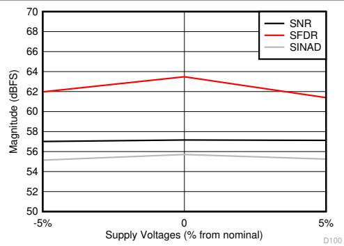
图 8-60. SNR, SFDR and SINAD vs Supply Voltage
