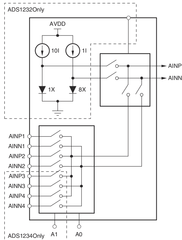
图 8-1. Measurement of the Temperature Sensor in the Input Multiplexer
