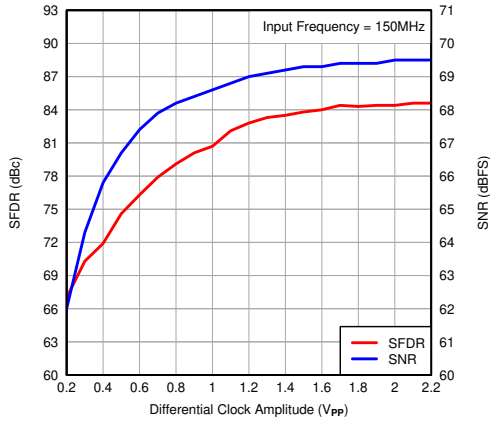
图 7-122. Performance vs Input Clock Amplitude
