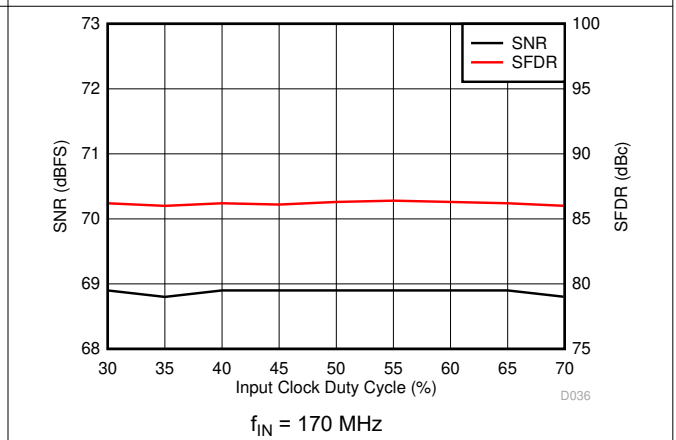
图 7-42. Performance vs Input Clock Duty Cycle
