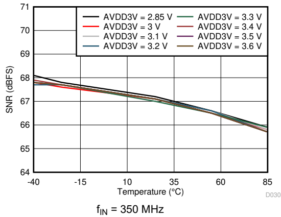
图 7-33. Signal-to-Noise Ratio vs AVDD3V Supply and Temperature
