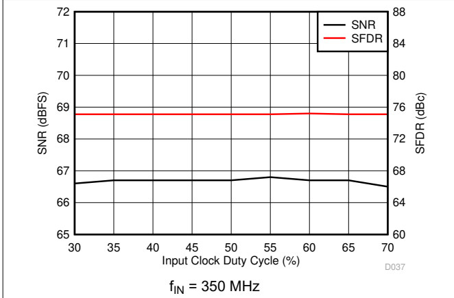
图 7-43. Performance vs Input Clock Duty Cycle
