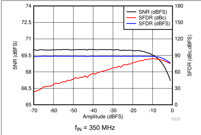
图 7-39. Performance vs Input Amplitude
