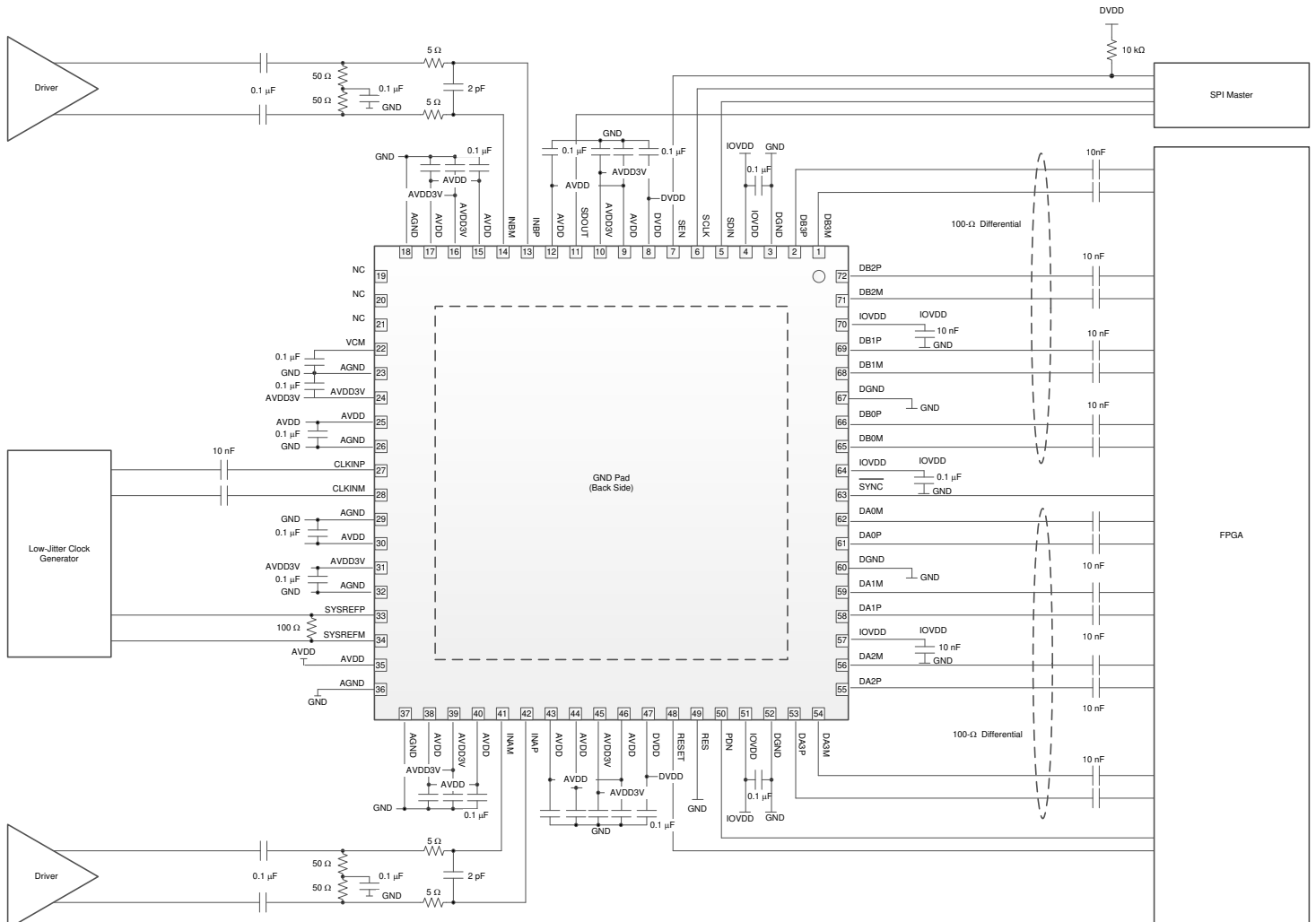
Figure 9-14. AC-Coupled Receiver
