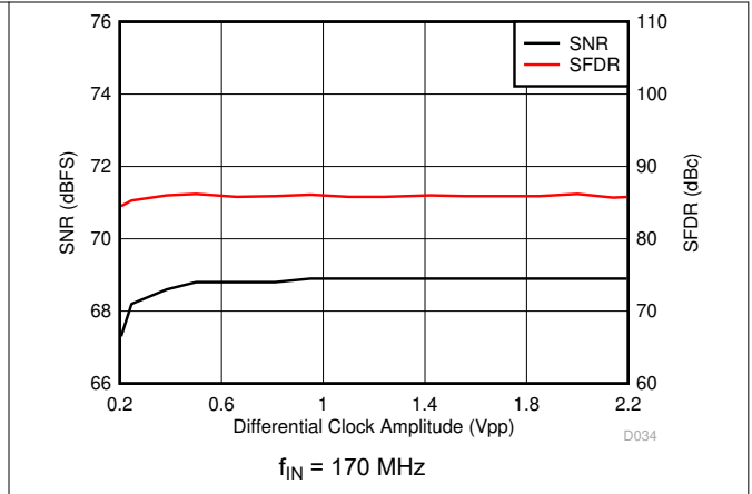
图 7-40. Performance vs Sampling Clock Amplitude
