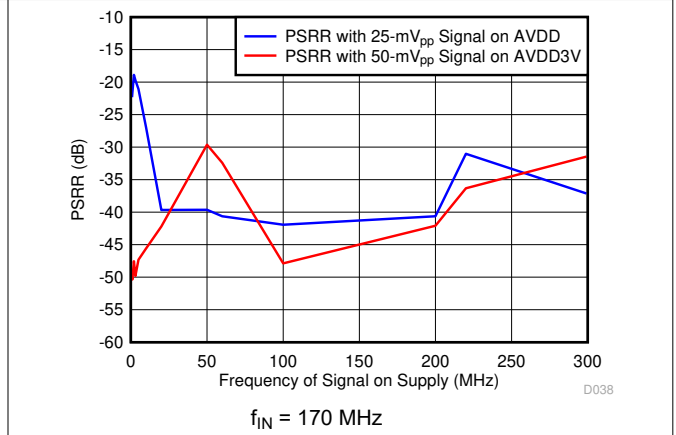
图 7-44. Power-Supply Rejection Ratio vs Test Signal Frequency
