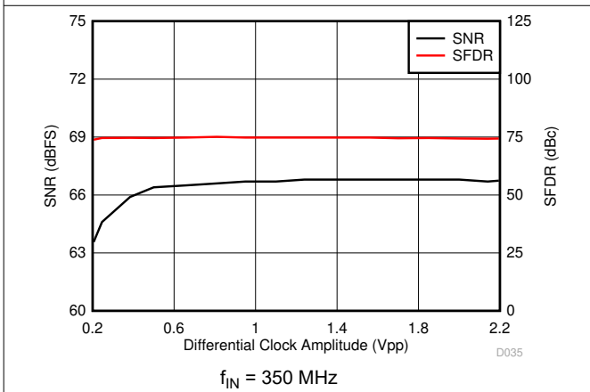
图 7-41. Performance vs Sampling Clock Amplitude
