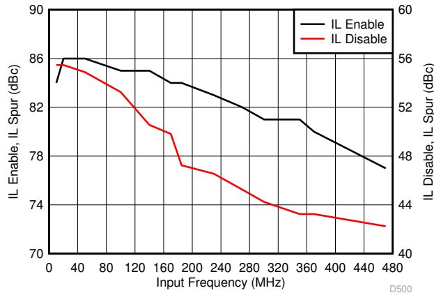
图 7-21. IL Spur vs Input Frequency
