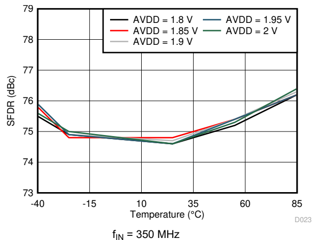
图 7-26. Spurious-Free Dynamic Range vs AVDD Supply and Temperature
