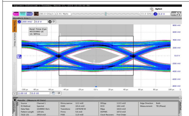
图 8-25. Eye at 10-Gbps Bit Rate with Default Output Swing
