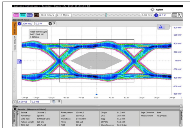
图 8-23. Eye at 5-Gbps Bit Rate with Default Output Swing
