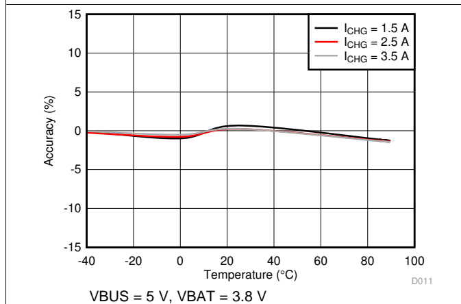
图 5. Charge Current Accuracy vs Temperature
