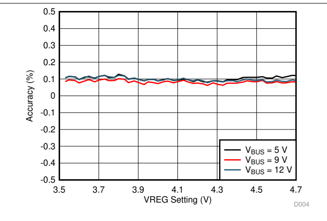
图 6. Battery Voltage Regulation Accuracy vs I²C VREG Setting
