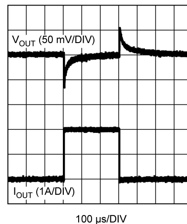
Figure 48. Transient Response
