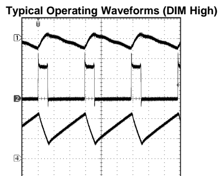
V_{IN} = 3.6V , 4 LEDs, I_{LED} = 30mA , V_{OUT} = 15.8V Channel 1: V_{OUT} (AC Coupled, 100mV/div) Channel 2: V_{SW} (DC Coupled, 10V/div) Channel 4: I_L (DC Coupled, 100mA/div) Time Base: 400ns/div
