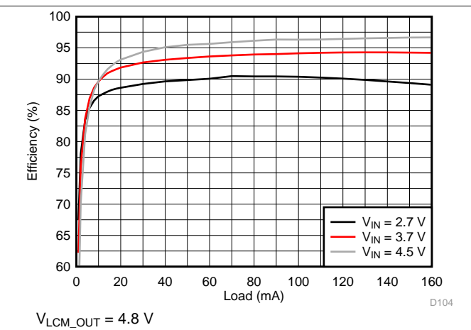
图 118. LCM Boost Efficiency
