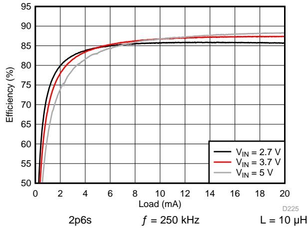
图 93. Backlight Boost Efficiency
