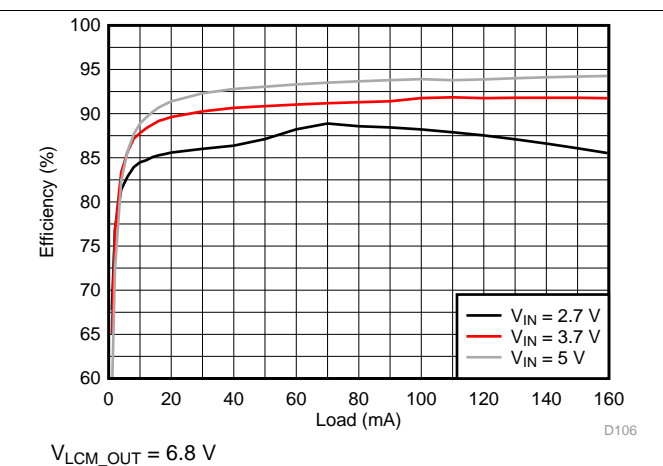
图 120. LCM Boost Efficiency
