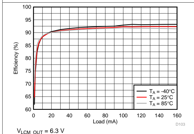
图 117. LCM Boost Efficiency
