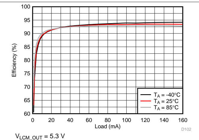
图 116. LCM Boost Efficiency
