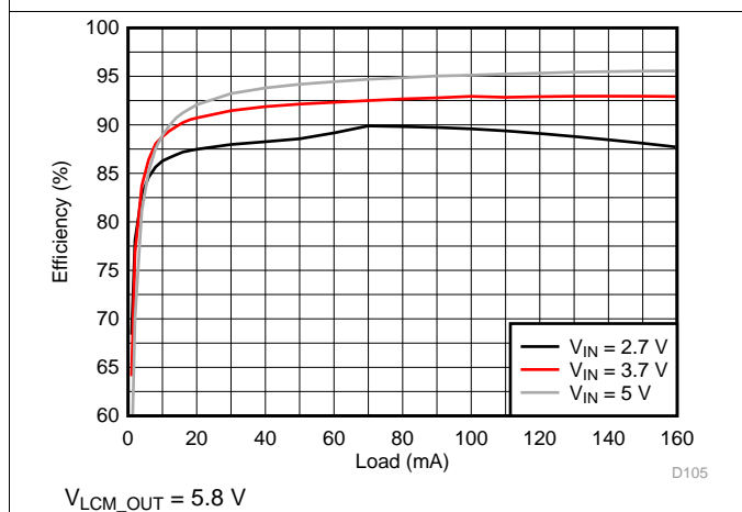
图 119. LCM Boost Efficiency
