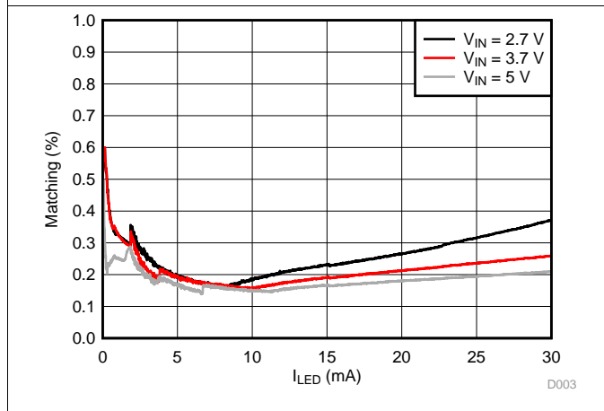
图 4. Backlight LED Current Matching
