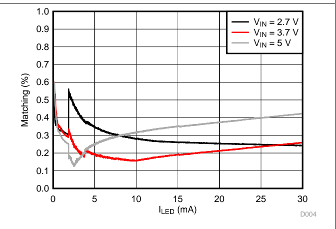
图 5. Backlight LED Current Matching
