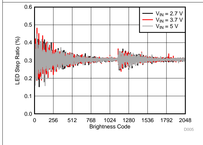
图 6. Backlight LED Current-Step Ratio
