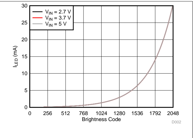
图 3. Backlight LED Current, Exponential Control
