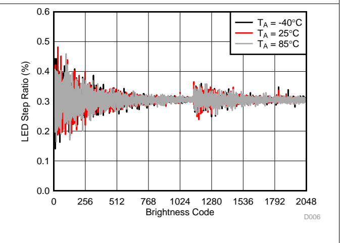
图 7. Backlight LED Current-Step Ratio
