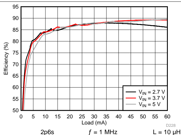
图 96. Backlight System Efficiency
