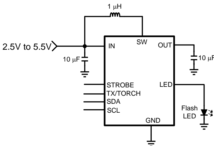
Figure 17. Typical Application Circuit
