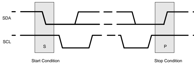
Figure 13. Start and Stop Conditions
