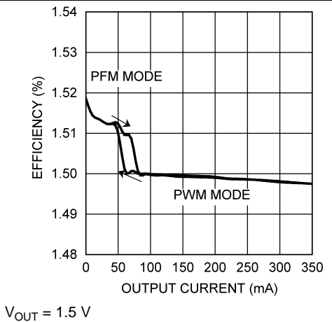
Figure 9. Output Voltage vs. Output Current
