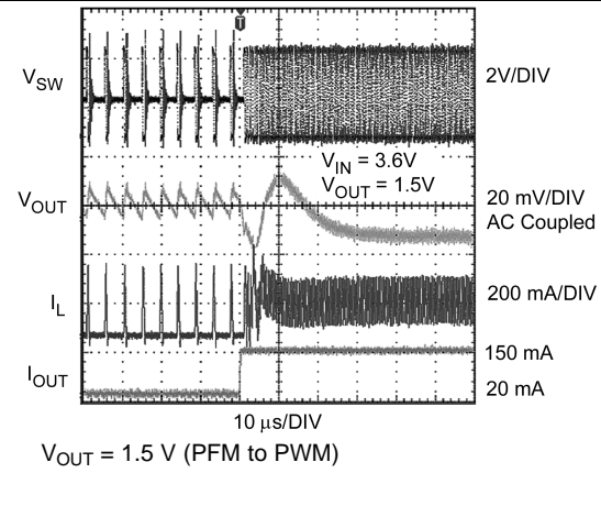
Figure 10. Mode Change by Load Transients
