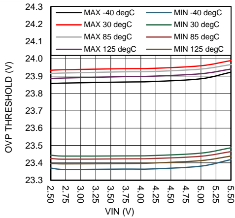
Figure 2. OVP Hysteresis
