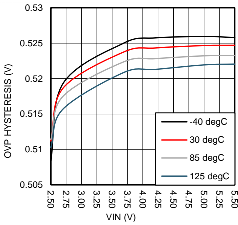
Figure 2. OVP Hysteresis
