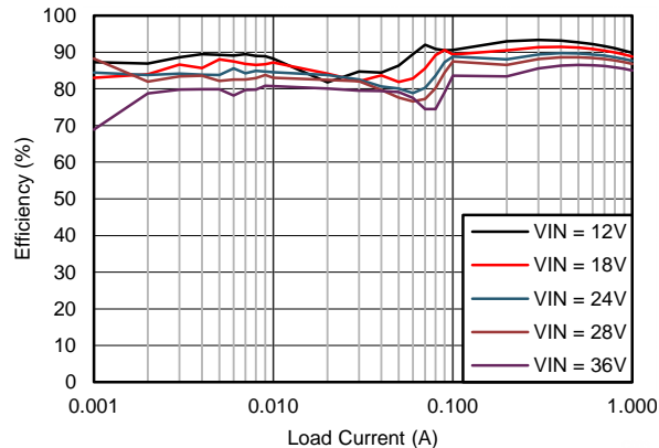
Figure 60. Efficiency
