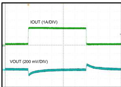
Figure 75. Output Voltage Regulation
