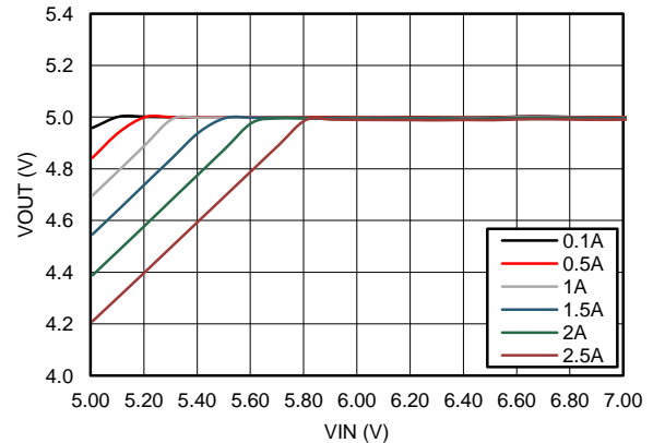
Figure 76. Dropout Curve
