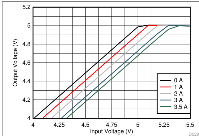
图 8-11. Overall Dropout Characteristics ( V_{OUT} = 5 V)
