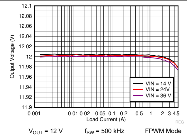
图 9-34. LM73605-Q1 Load and Line Regulation
