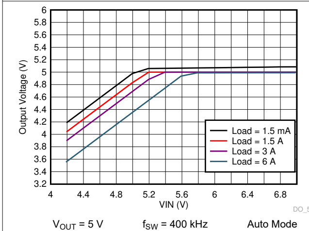
图 9-35. LM73606-Q1 Dropout Curve
