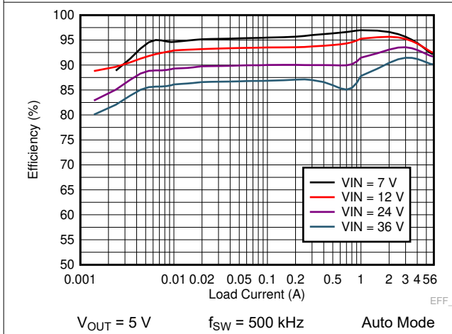
图 9-13. LM73606-Q1 Efficiency
