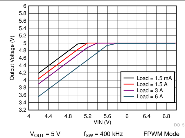
图 9-36. LM73606-Q1 Dropout Curve
