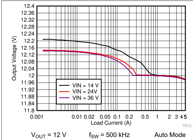
图 9-33. LM73605-Q1 Load and Line Regulation
