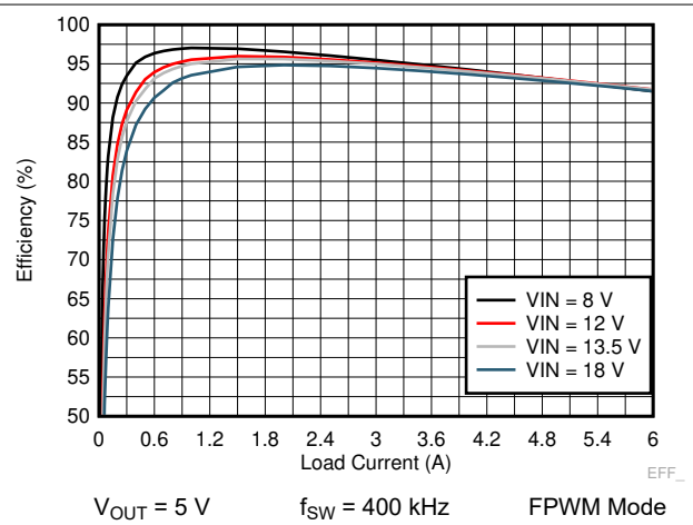
图 9-12. LM73606-Q1 Efficiency
