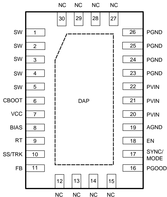
RNP Package 30-Pin Wettable Flanks QFN (WQFN) 6 mm × 4 mm × 0.8 mm Top View
