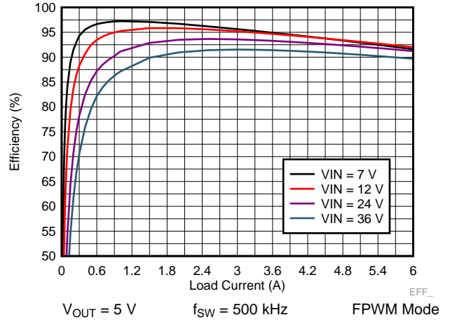
图 34. LM73606 Efficiency
