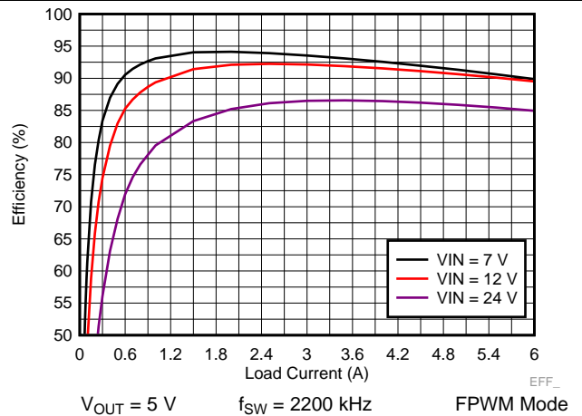
图 38. LM73606 Efficiency
