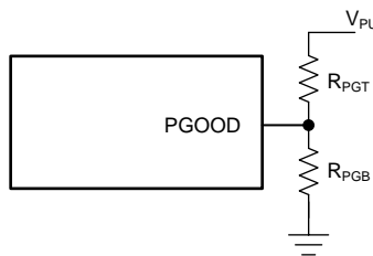
图 24. Divider for PGOOD Pullup Voltage
