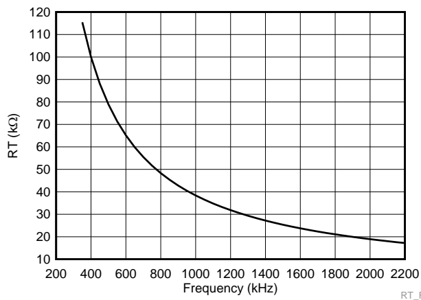
图 21. R_T Resistance vs Switching Frequency
