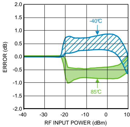
Figure 39. Temperature Variation (50 Units) vs. RF Input Power at 5800 MHz
