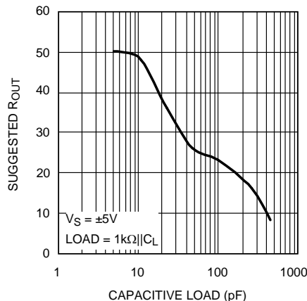
Figure 20. Suggested R_{OUT} vs. C_L
