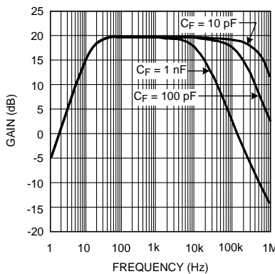
Figure 51. Frequency Response of the Inverting Audio Preamplifier
