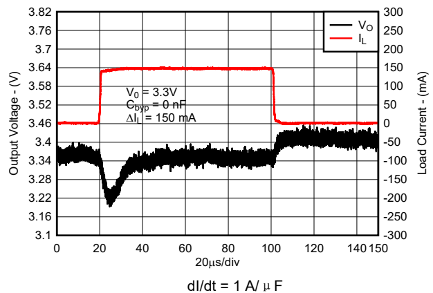
图 8-12. Load Transient Response for New Chip
