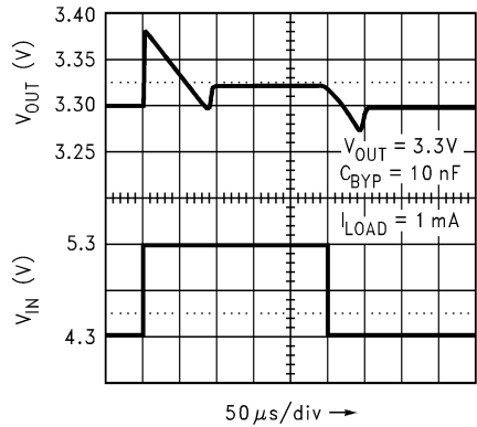
图 8-17. Line Transient Response for Legacy Chip
