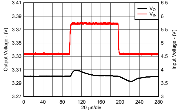
图 8-14. Line Transient Response for New Chip
