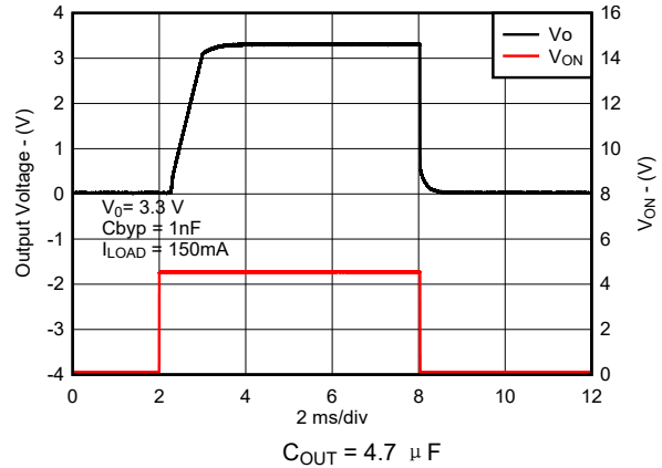
图 8-26. Turn-On Time for New Chip
