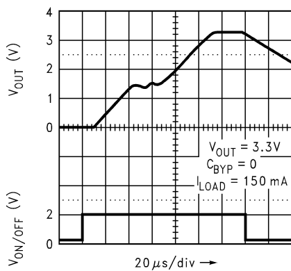
图 8-21. Turn-On Time for Legacy Chip
