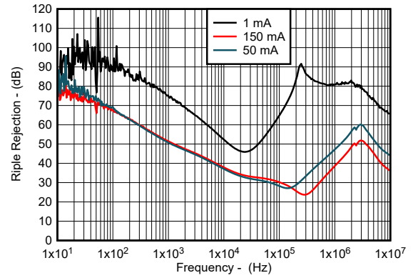
图 6-14. Ripple Rejection vs Frequency for New Chip
