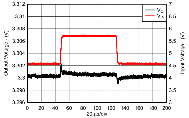
图 8-20. Line Transient Response for New Chip
