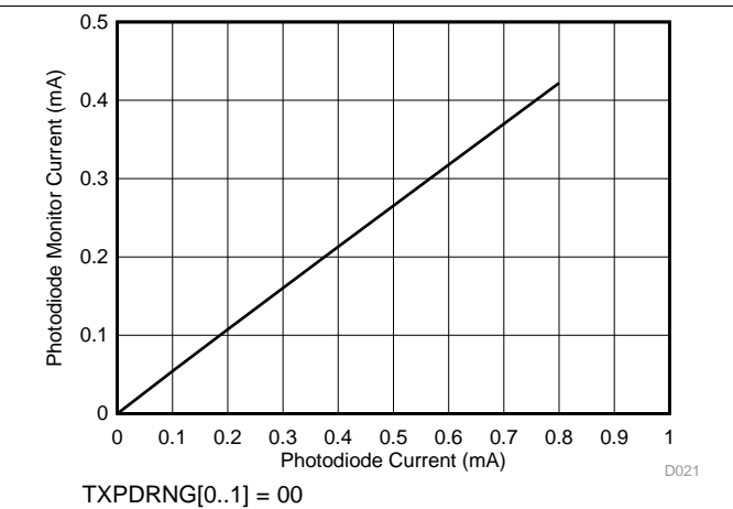
Figure 13. Photodiode-Monitor Current I_{(MONP)} vs PD Current
