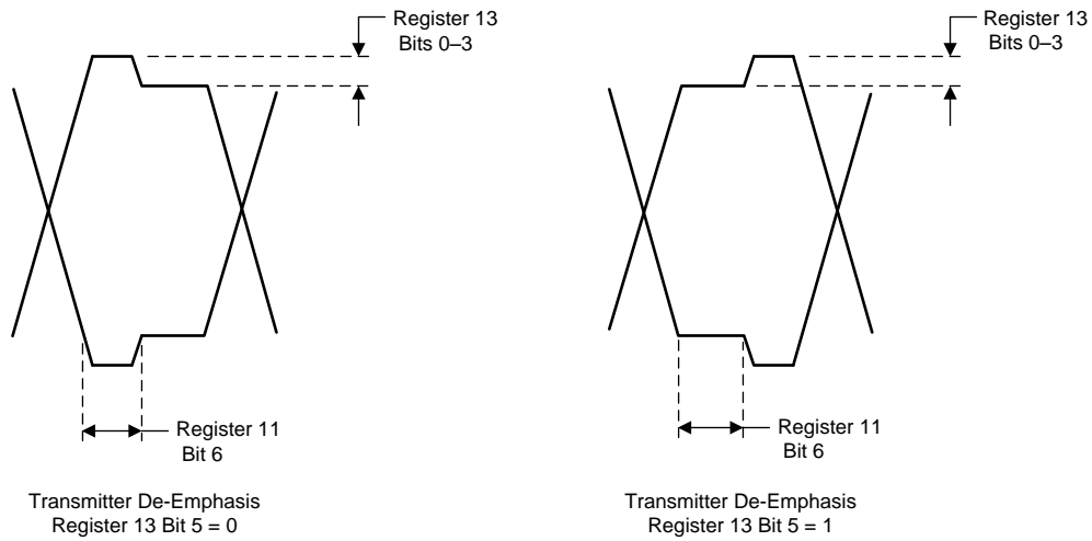
图 34. Transmitter De-Emphasis Modes
