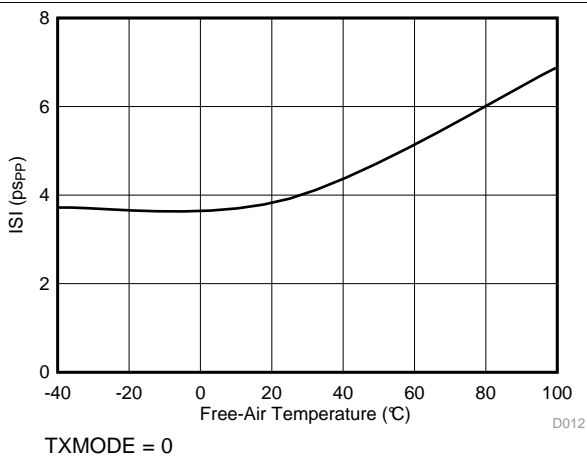
Figure 4. TX Deterministic Jitter vs Temperature
