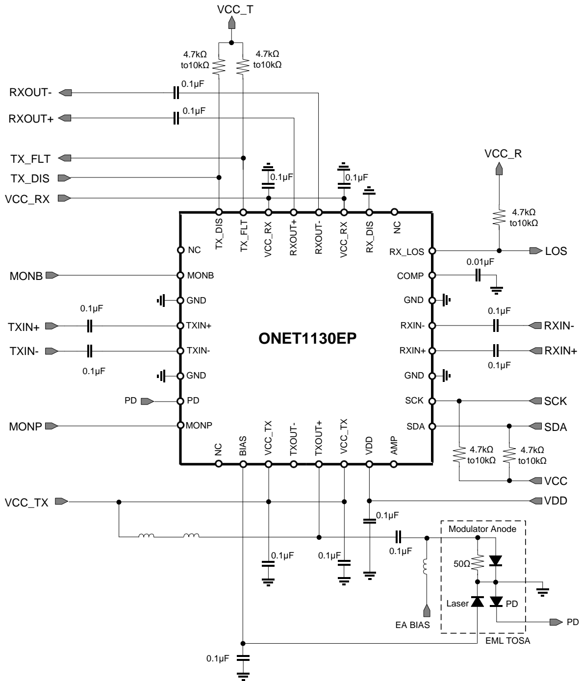
图 66. Typical Application Circuit in Single-Ended Mode with an EML and the PD Monitor Cathode Available
