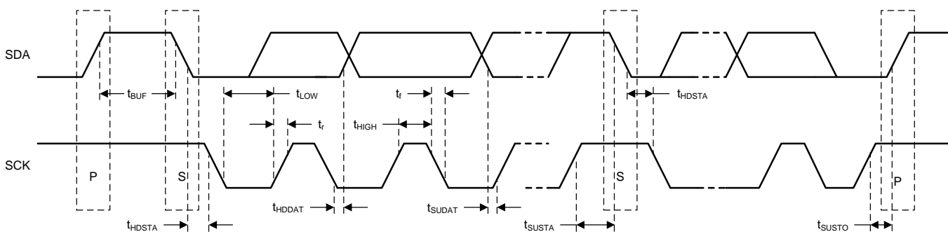
图 1. 2-Wire Interface Diagram
