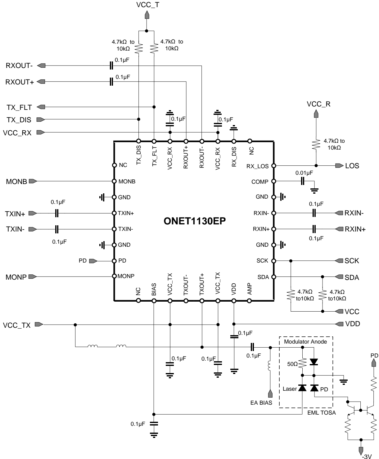
图 67. Typical Application Circuit in Single-Ended Mode with an EML and the PD Monitor Anode Available
