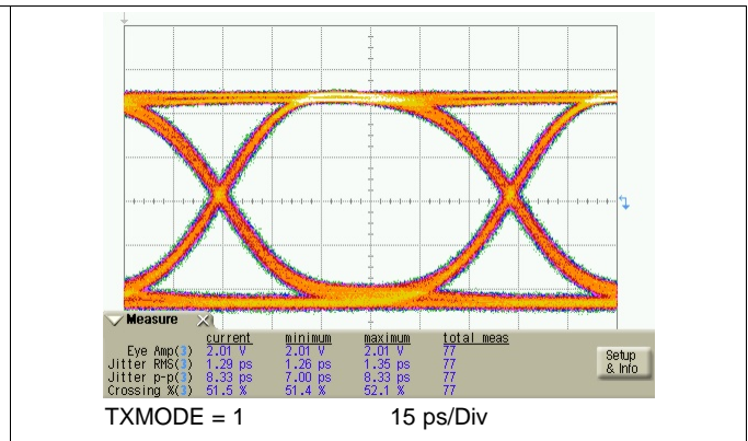
Figure 21. TX Eye-Diagram at 11.3 Gbps
