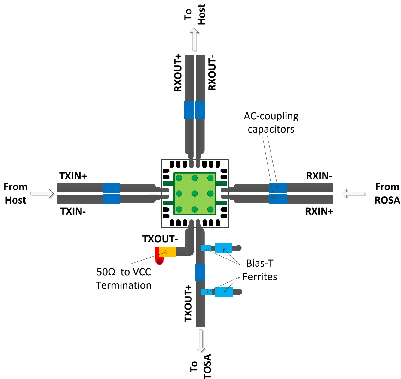
图 69. Board Layout
