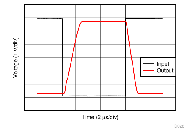
图 7-30. Overload Recovery
